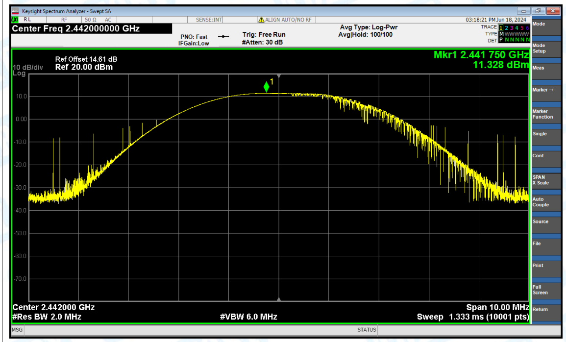
Power NVNT 2442MHz Ant1
