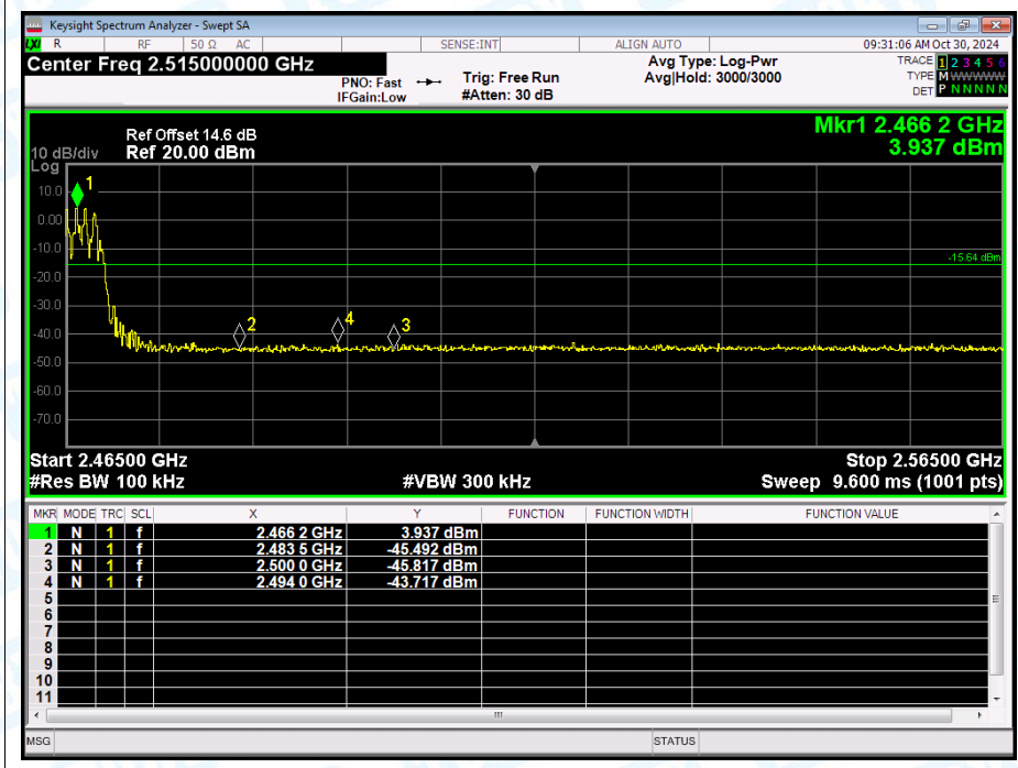
Band Edge(Hopping) NVNT 2469MHz Hopping Emission
