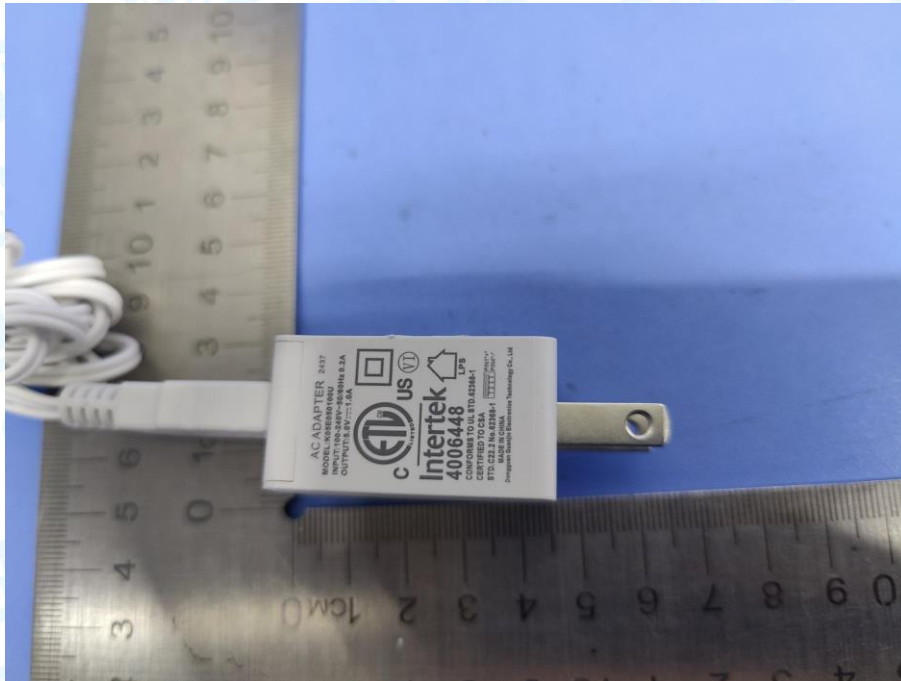
Photo 12 Adapter Appearance 5#
