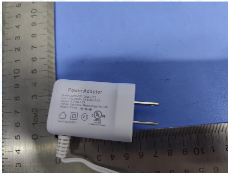
Photo 10 Adapter Appearance 3#
