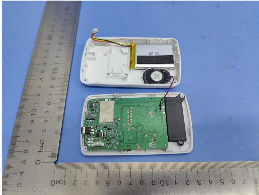
Photo 13 Internal of EUT (Differential prototype)
