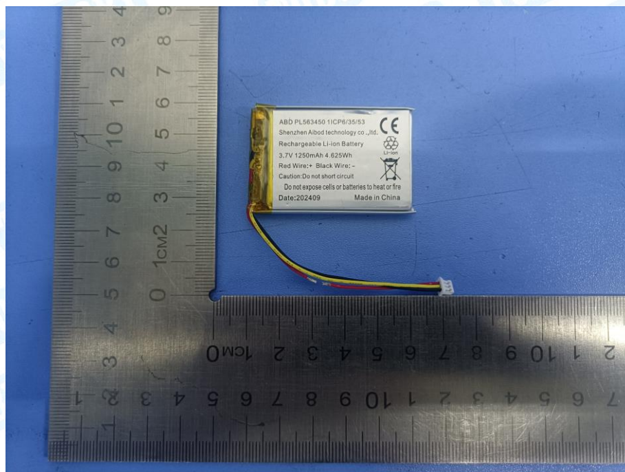
Photo 19 Battery Appearance (ABD PL563450)
