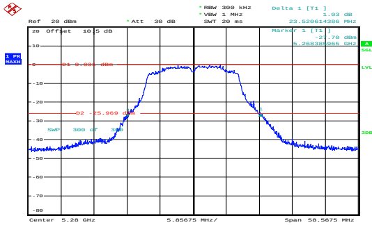
a_5280MHz_Chain 0 23.521MHz
