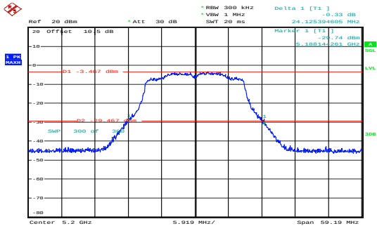
n20_5200MHz_Chain 0 24.125MHz
