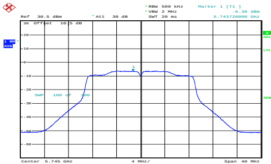
n20_5745MHz_Chain 0 -6.38dBm/MHz
