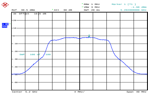
n20_5200MHz_Chain 0 -1.98dBm/MHz
