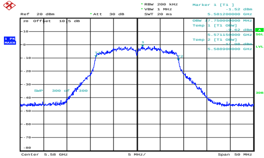
n20_5580MHz_Chain 0 17.750MHz
