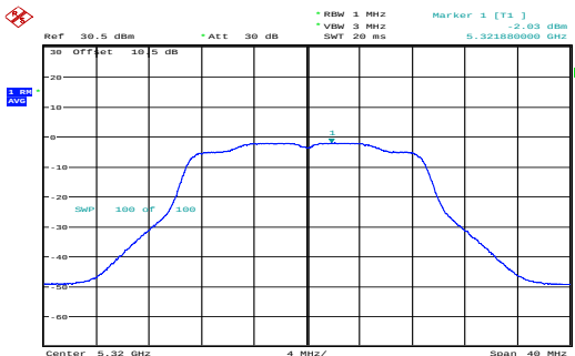
n20_5320MHz_Chain 1 -2.03dBm/MHz
