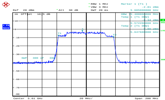
ac80_5610MHz_Chain 0 75.400MHz
