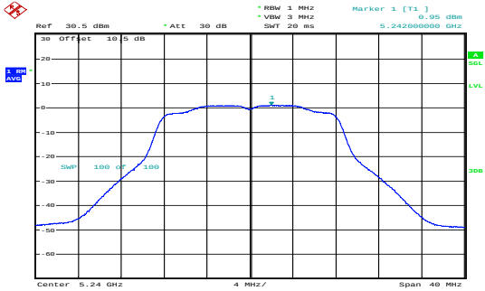
a_5240MHz_Chain 0 0.95dBm/MHz
