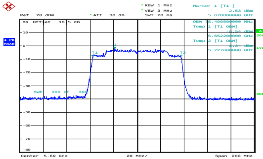
ac80_5690MHz_Chain 0 75.400MHz
