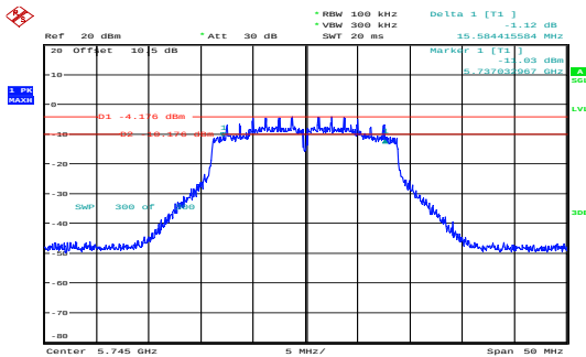
n20_5745MHz_Chain 0 15.584MHz
