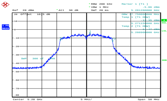
n20_5280MHz_Chain 0 17.750MHz
