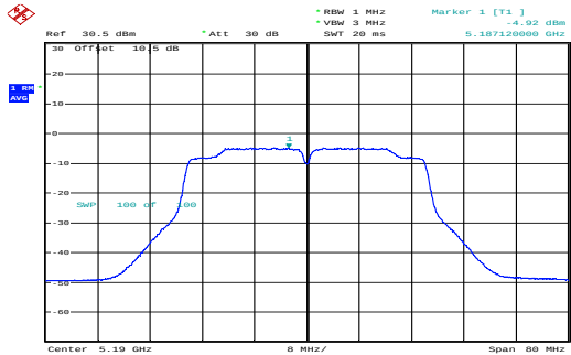
n40_5190MHz_Chain 1 -4.92dBm/MHz
