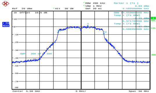
a_5580MHz_Chain 0 16.650MHz
