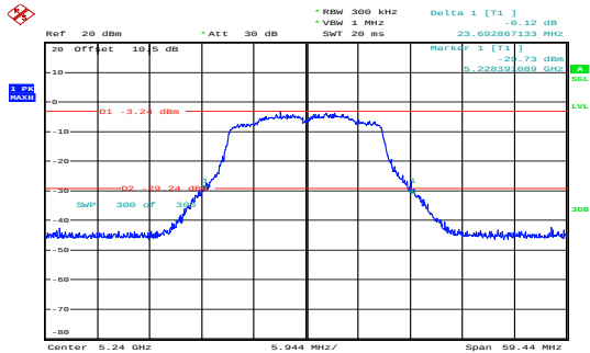
n20_5240MHz_Chain 0 23.693MHz
