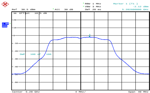
n20_5280MHz_Chain 0 -2.12dBm/MHz
