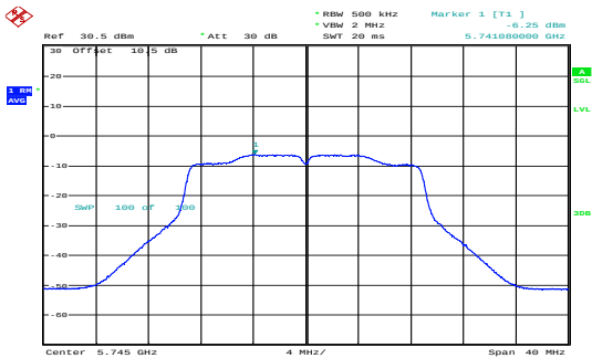
n20_5745MHz_Chain 1 -6.25dBm/MHz
