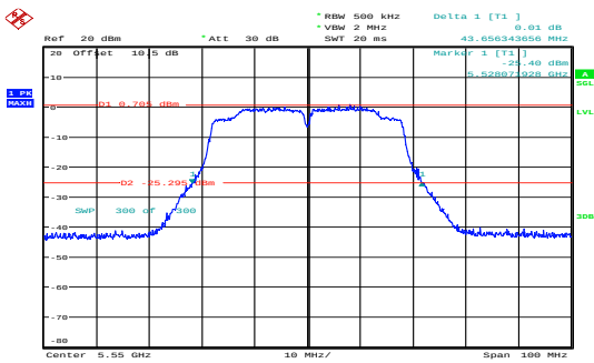
n40_5550MHz_Chain 0 43.656MHz
