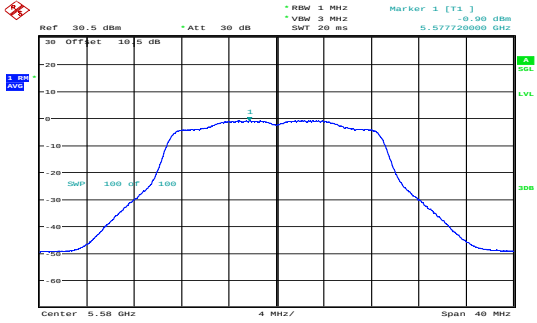
n20_5580MHz_Chain 1 -0.90dBm/MHz
