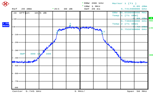
a_5745MHz_Chain 0 16.650MHz
