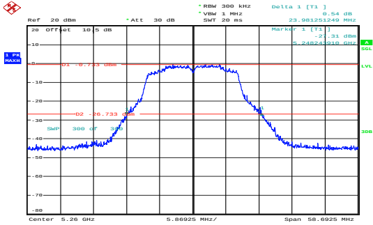
a_5260MHz_Chain 0 23.981MHz
