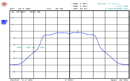
n20_5200MHz_Chain 1 -2.07dBm/MHz
