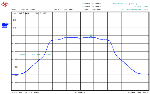
n20_5180MHz_Chain 1 -2.03dBm/MHz
