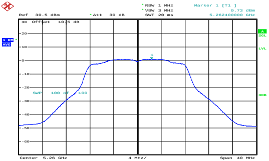
a_5260MHz_Chain 1 0.73dBm/MHz
