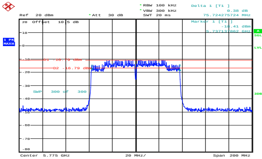
ac80_5775MHz_Chain 0 75.724MHz
