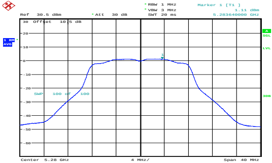
a_5280MHz_Chain 0 1.11dBm/MHz
