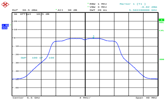
n20_5500MHz_Chain 1 -0.82dBm/MHz
