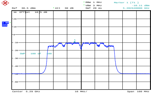
ac80_5290MHz_Chain 0 -10.11dBm/MHz
