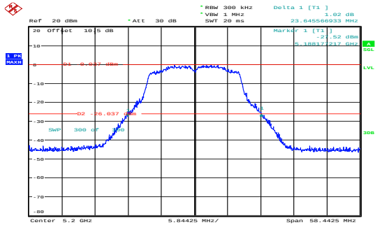
a_5200MHz_Chain 0 23.646MHz
