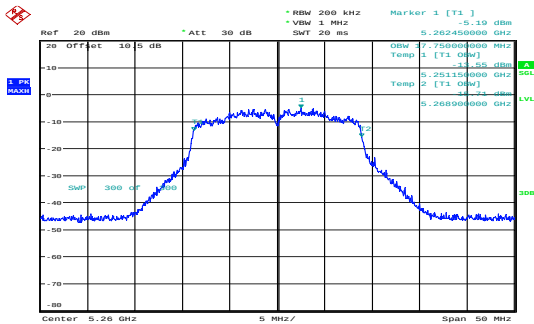
n20_5260MHz_Chain 0 17.750MHz
