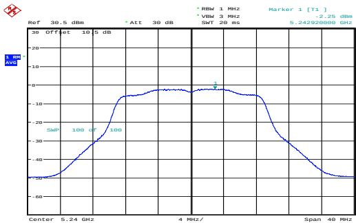
n20_5240MHz_Chain 0 -2.25dBm/MHz
