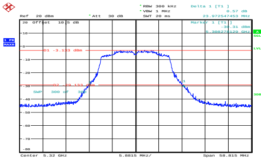
n20_5320MHz_Chain 0 23.973MHz
