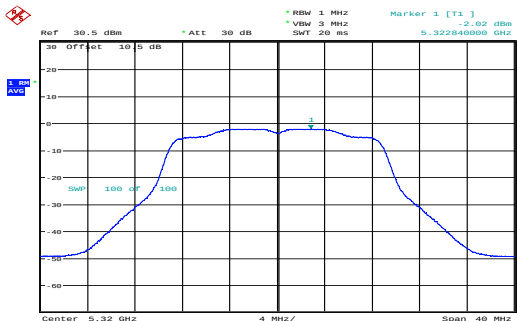
n20_5320MHz_Chain 0 -2.02dBm/MHz
