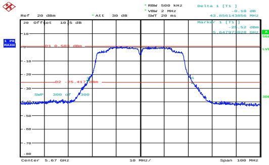
n40_5670MHz_Chain 0 43.856MHz
