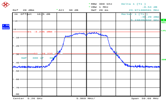
n20_5260MHz_Chain 0 23.971MHz
