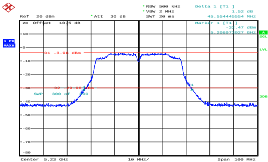
n40_5230MHz_Chain 0 45.554MHz
