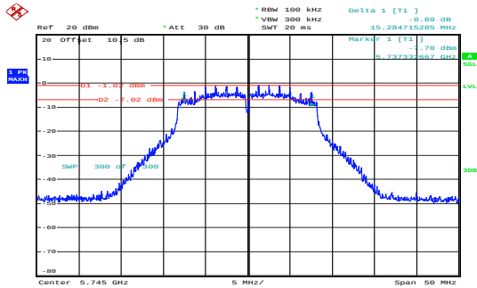
a_5745MHz_Chain 0 15.285MHz
