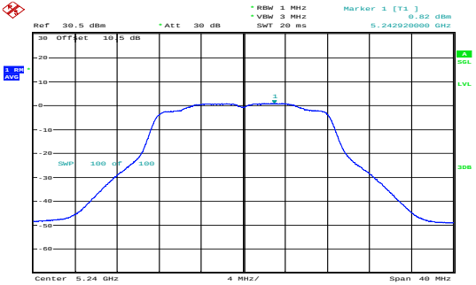
a_5240MHz_Chain 1 0.82dBm/MHz
