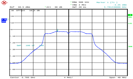
a_5785MHz_Chain 1 -3.25dBm/MHz
