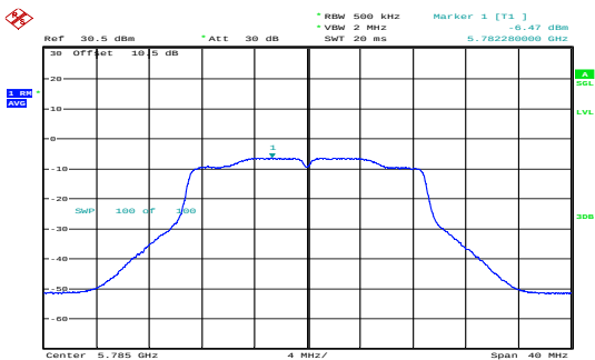
n20_5785MHz_Chain 1 -6.47dBm/MHz
