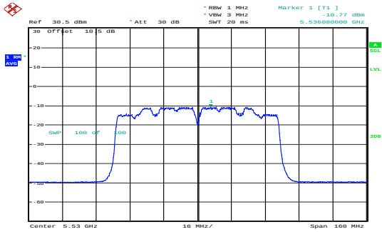
ac80_5530MHz_Chain 0 -10.77dBm/MHz
