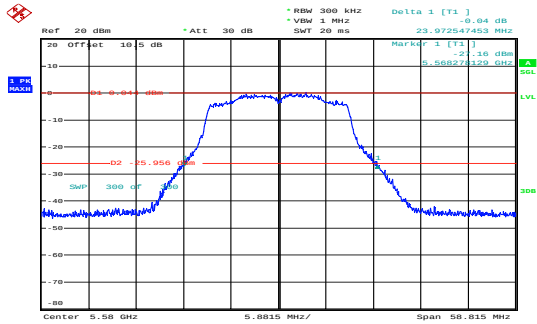
n20_5580MHz_Chain 0 23.973MHz
