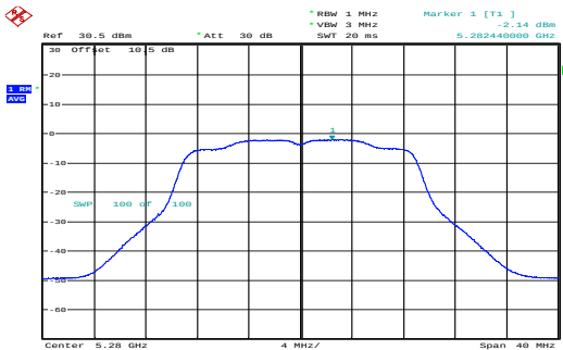
n20_5280MHz_Chain 1 -2.14dBm/MHz
