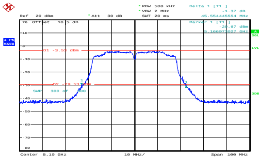
n40_5190MHz_Chain 0 45.554MHz
