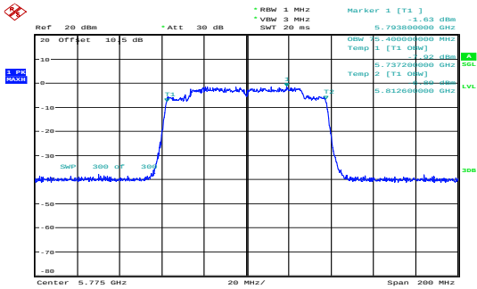
ac80_5775MHz_Chain 0 75.400MHz
