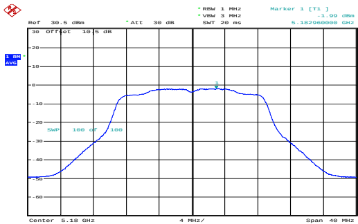
n20_5180MHz_Chain 0 -1.99dBm/MHz
