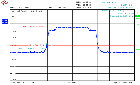
ac80_5290MHz_Chain 0 82.917MHz
