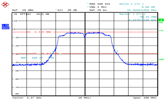
n40_5270MHz_Chain 0 44.356MHz
