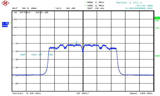
ac80_5690MHz_Chain 0 -11.31dBm/MHz
