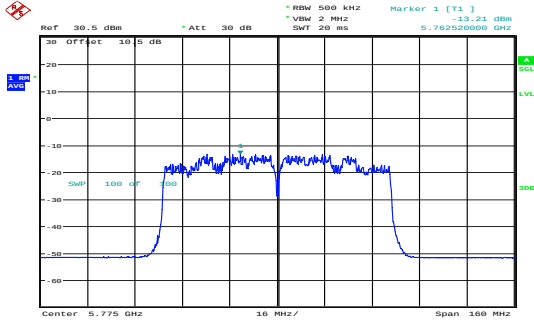
ac80_5775MHz_Chain 0 -13.21dBm/MHz
