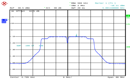
n40_5795MHz_Chain 0 -10.11dBm/MHz
