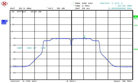
n40_5795MHz_Chain 1 -10.02dBm/MHz
