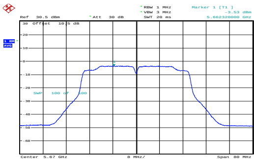
n40_5670MHz_Chain 0 -3.53dBm/MHz
