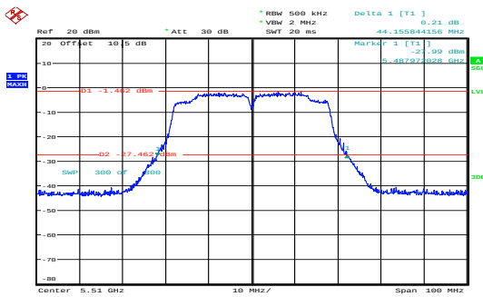
n40_5510MHz_Chain 0 44.156MHz
