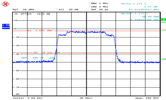
ac80_5690MHz_Chain 0 82.517MHz
