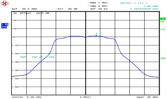
a_5280MHz_Chain 1 1.00dBm/MHz
