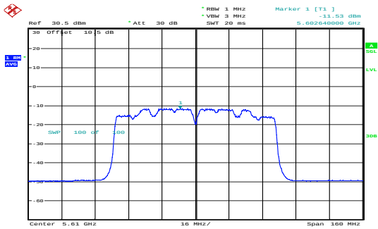
ac80_5610MHz_Chain 0 -11.53dBm/MHz
