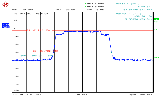
ac80_5610MHz_Chain 0 82.517MHz
