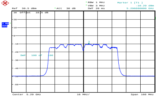
ac80_5290MHz_Chain 1 -10.29dBm/MHz
