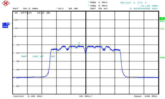
ac80_5690MHz_Chain 1 -11.29dBm/MHz
