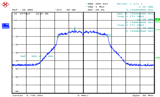
n20_5745MHz_Chain 0 17.750MHz
