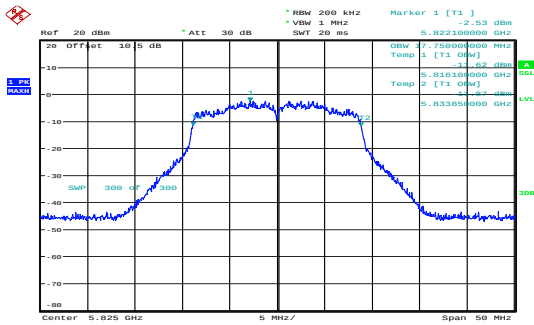
n20_5825MHz_Chain 0 17.750MHz
