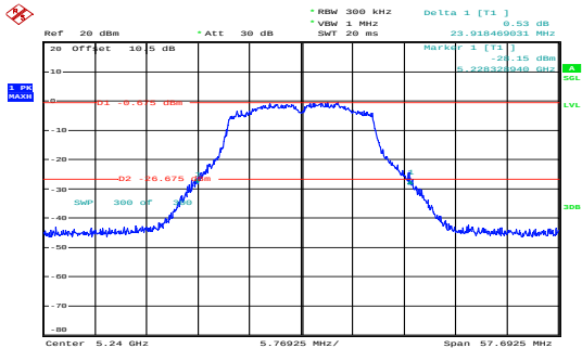
a_5240MHz_Chain 0 23.918MHz
