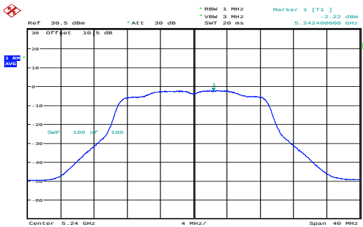
n20_5240MHz_Chain 1 -2.22dBm/MHz
