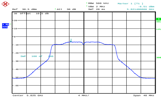
n20_5825MHz_Chain 0 -6.51dBm/MHz
