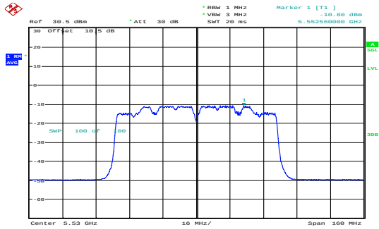
ac80_5530MHz_Chain 1 -10.80dBm/MHz
