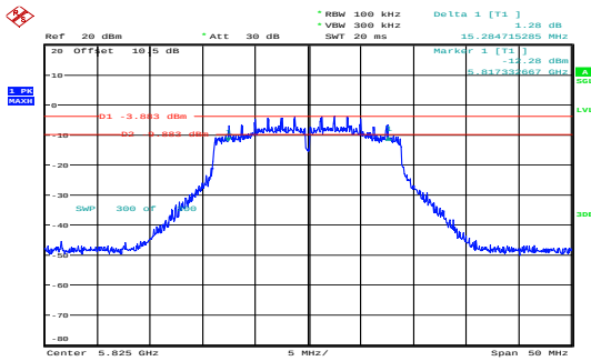
n20_5825MHz_Chain 0 15.285MHz
