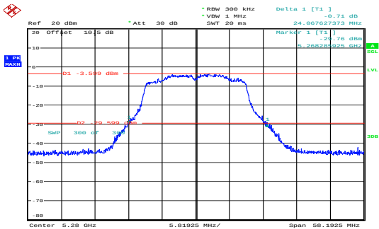
n20_5280MHz_Chain 0 24.068MHz
