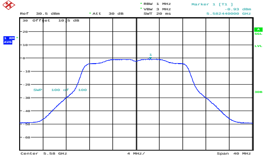
n20_5580MHz_Chain 0 -0.93dBm/MHz
