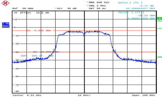
n40_5310MHz_Chain 0 43.157MHz
