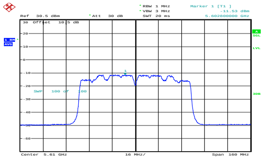
ac80_5610MHz_Chain 1 -11.53dBm/MHz
