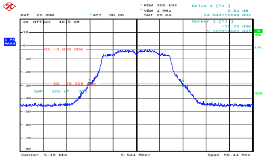
n20_5180MHz_Chain 0 24.049MHz
