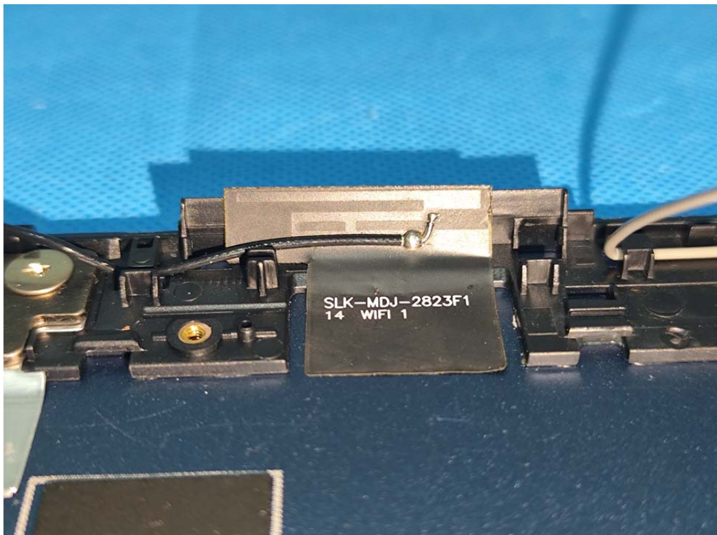
MAIN Antenna(Wi-Fi Chain 0)
