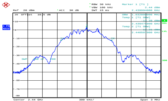
Middle 1.032MHz
