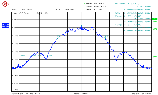
High 1.029MHz
