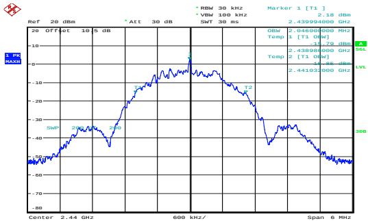
Middle 2.046MHz
