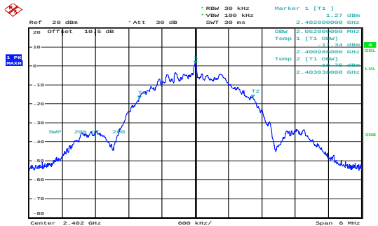
Low 2.052MHz
