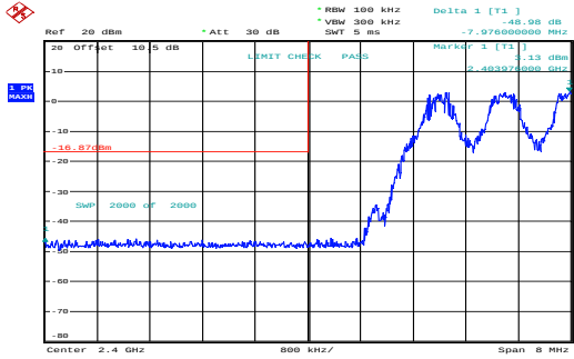
GFSK_Hopping_Lower 48.98dB
