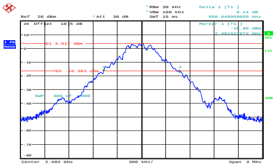
GFSK_Low 0.950MHz
