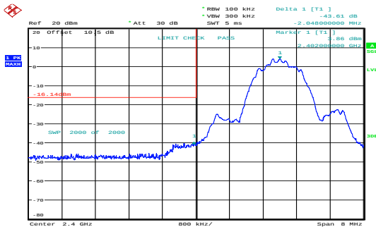
8DPSK_Low 43.61dB
