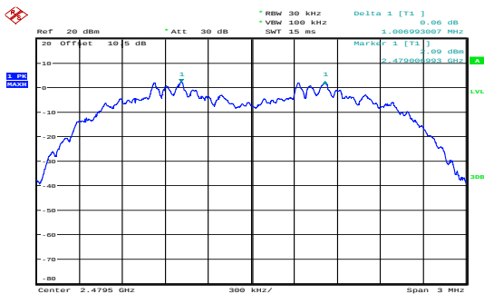
8DPSK_High 1.007MHz
