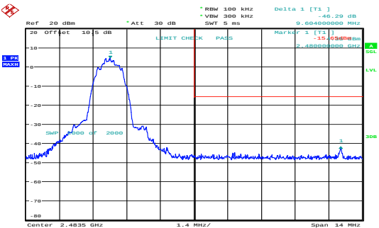
8DPSK_High 46.29dB
