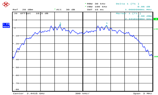
8DPSK_Middle 1.001MHz
