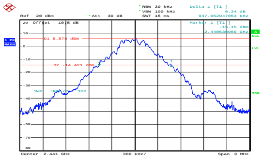
GFSK_Middle 0.947MHz
