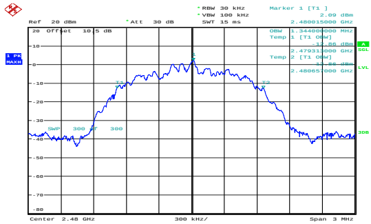
\pi/4 -DQPSK_High 1.344MHz
