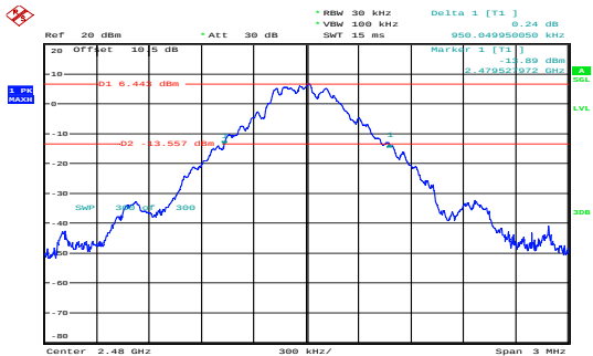
GFSK_High 0.950MHz
