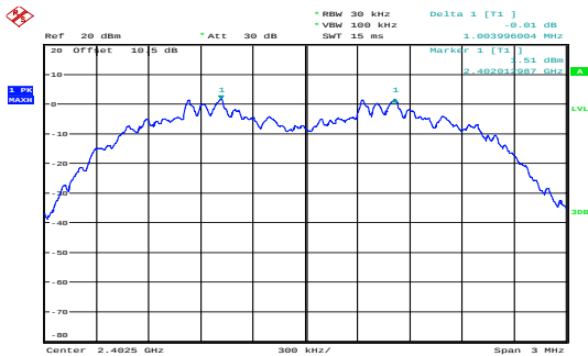
8DPSK_Low 1.004MHz
