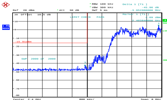
8DPSK_Hopping_Lower 45.96dB
