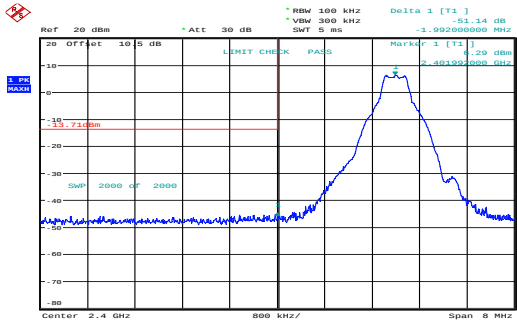
GFSK_Low 51.14dB
