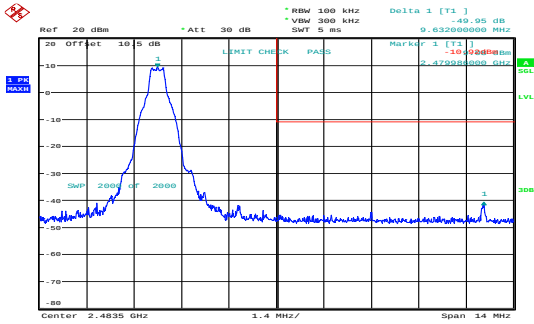
GFSK_High 49.95dB
