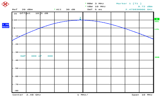
GFSK_High 9.72dBm
