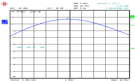
GFSK_Low 6.94dBm
