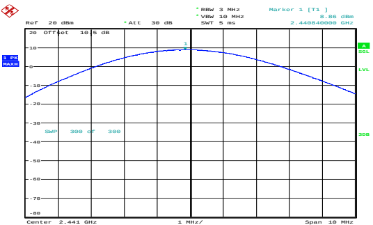
GFSK_Middle 8.86dBm
