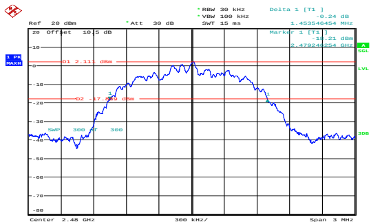
\pi/4 -DQPSK_High 1.454MHz
