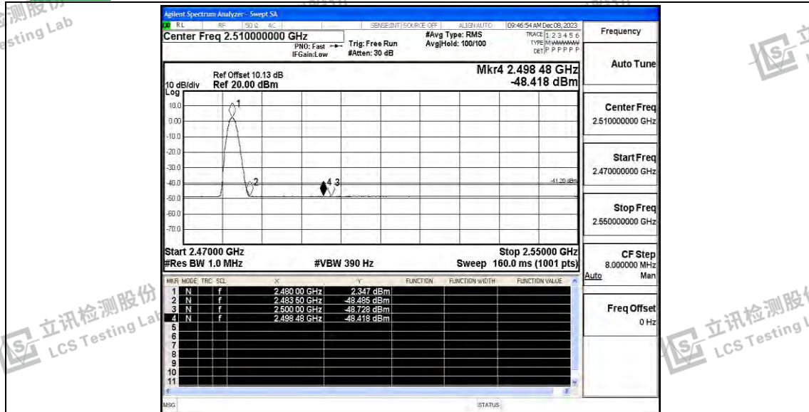
DH5_BT Ant_High_2480_Peak
