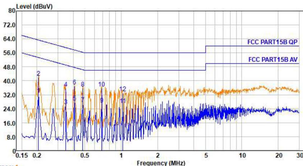
Trace: 1
