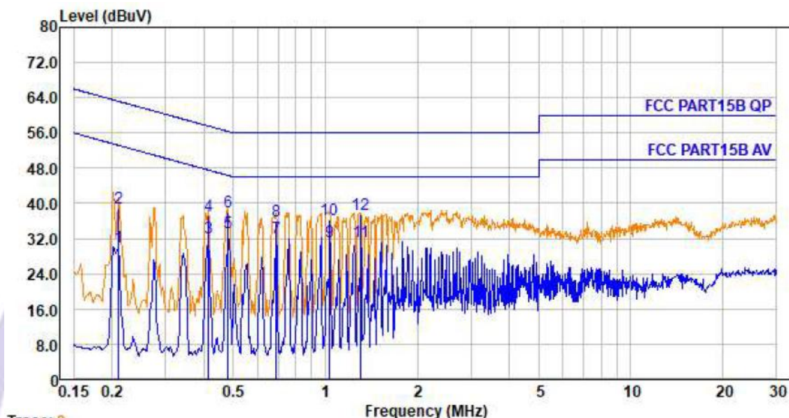
Trace: 3
