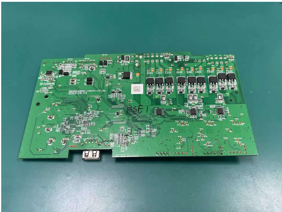
Internal: Bottom of main board
