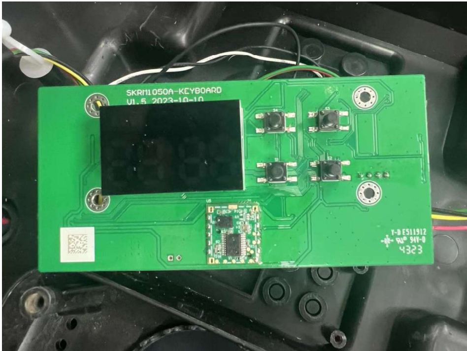
Internal: Top of display & key
