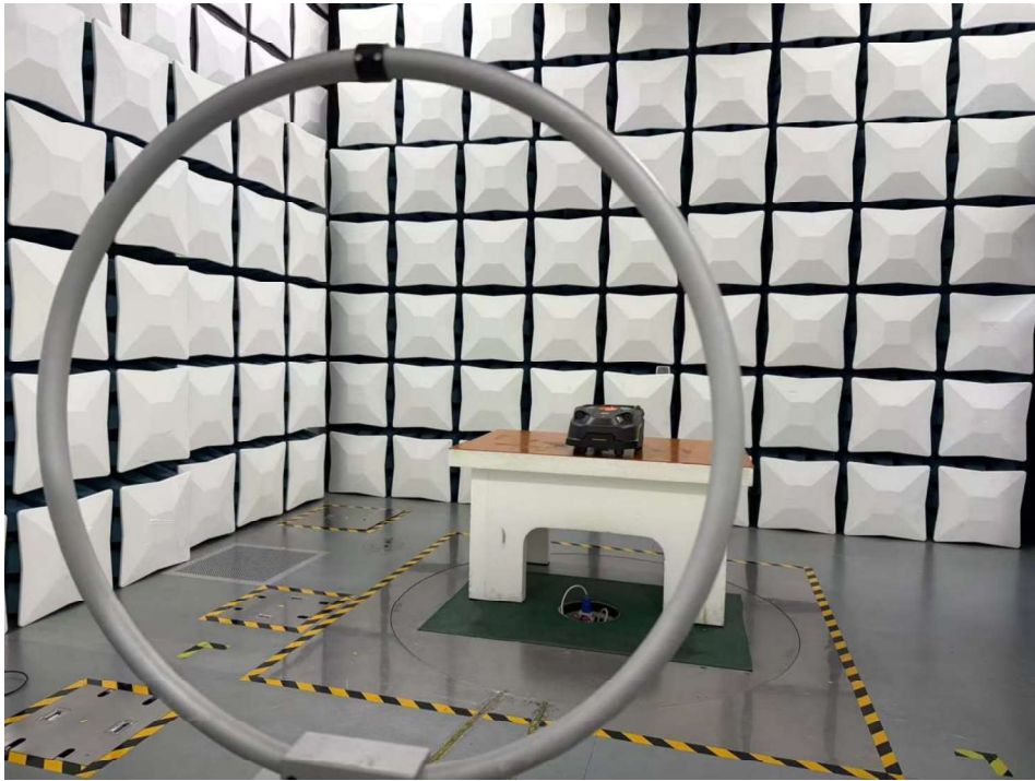
Test Set-up: Radiated spurious emission 9KHz-30MHz
