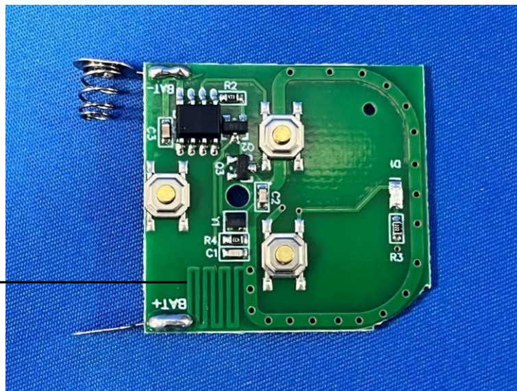
315MHz PCB Antenna
