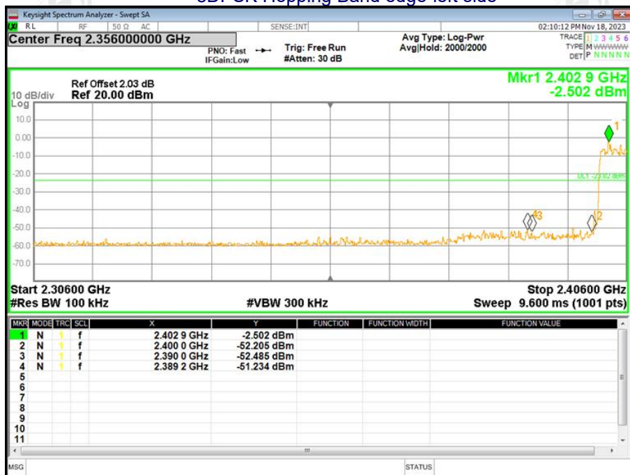
8DPSK Hopping Band edge-left side
