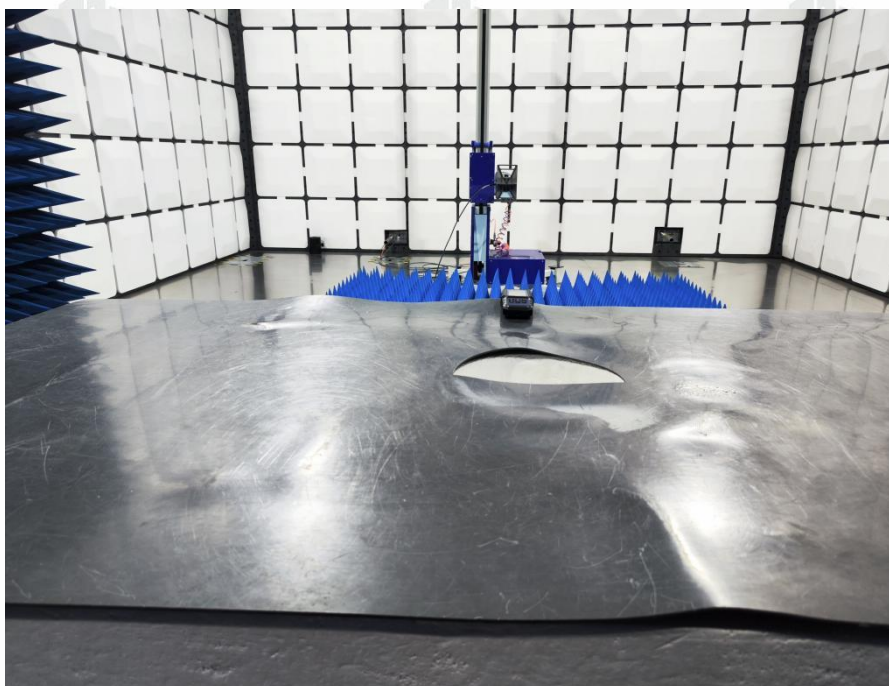
Radiated Emission (Above 1GHz)
