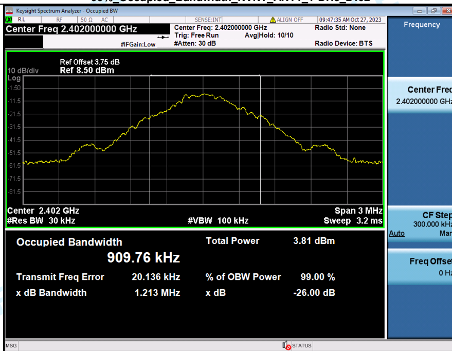
99%_Occupied_Bandwidth_NVNT_ANT1_1-DH5_2402
