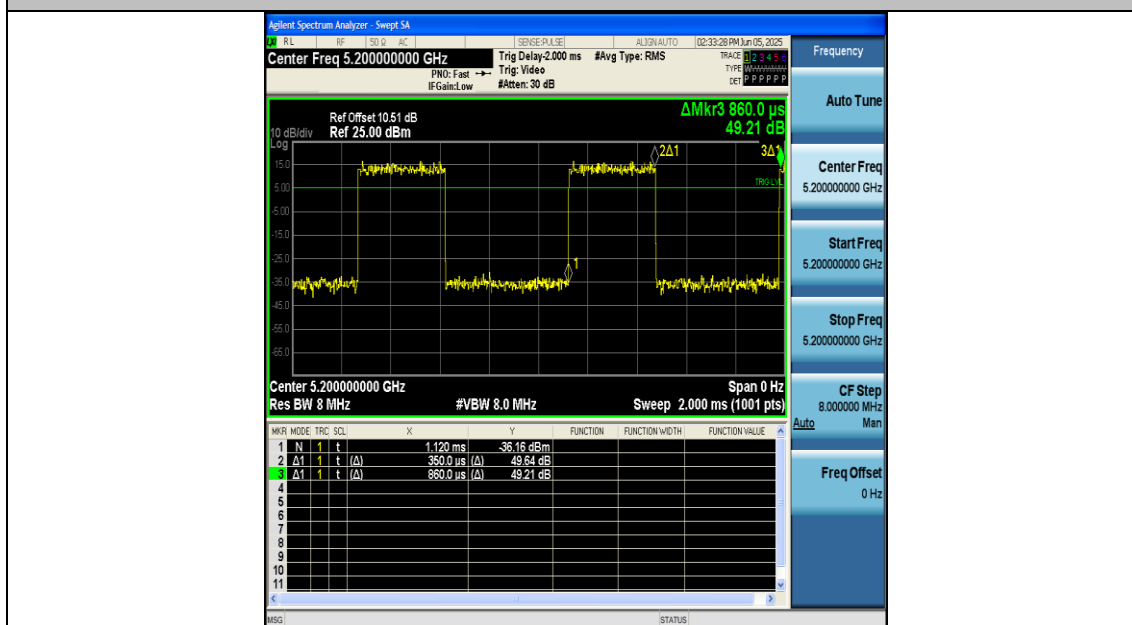
NTNV-11AC20MIMO-Ant2-5200
