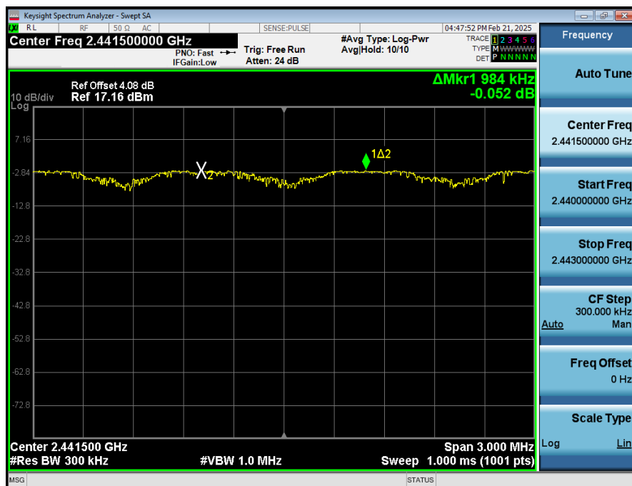
Carrier_Frequencies_Separation_(Hopping)_NVNT_ANT1_2-DH1_Hopping
