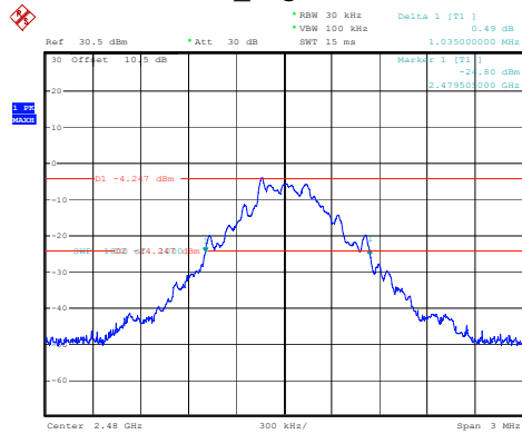
DH1_High 1.035MHz
