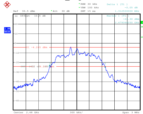
2DH1_High 1.313MHz
