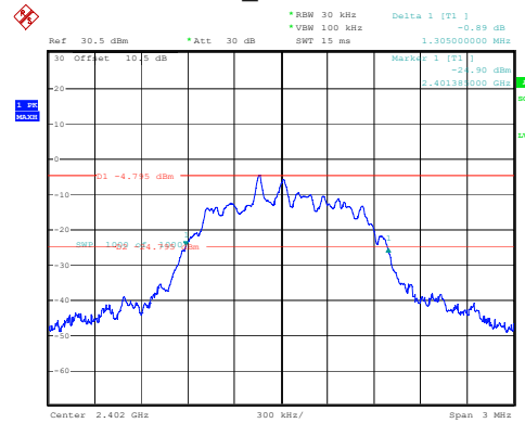
2DH1_Low 1.305MHz
