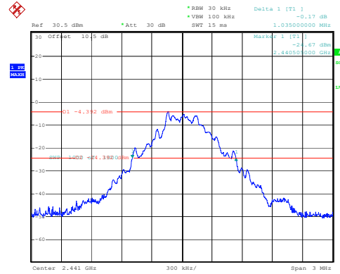
DH1_Middle 1.035MHz
