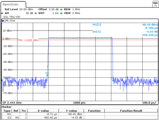
DH1_Hopping 0.420ms
