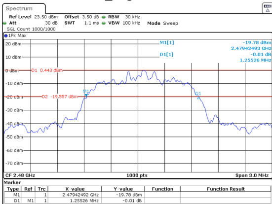
2DH1_High 1.255MHz
