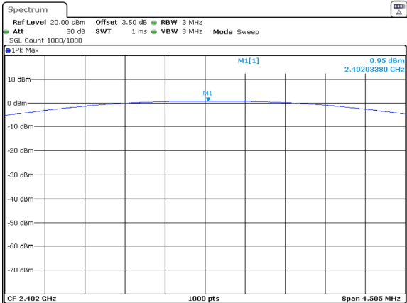
DH1_Low 0.95dBm
