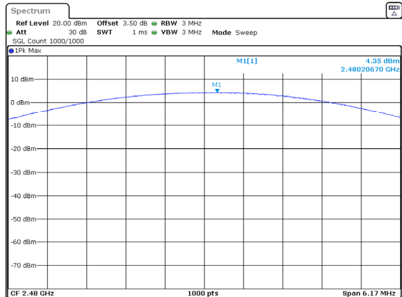
3DH1_High 4.35dBm
