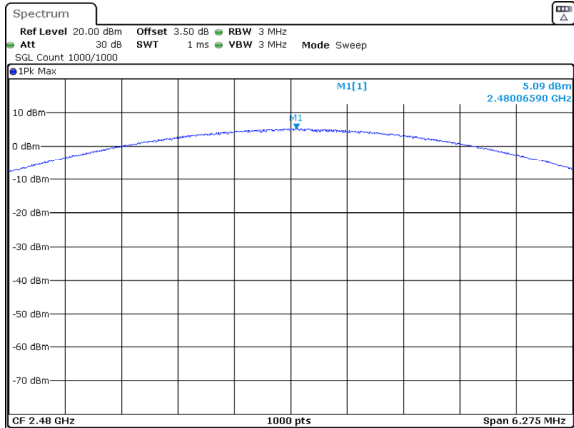
2DH1_High 5.09dBm
