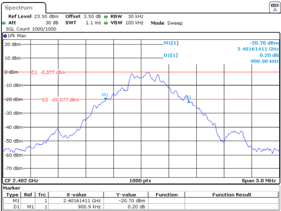
DH1_Low 0.901MHz
