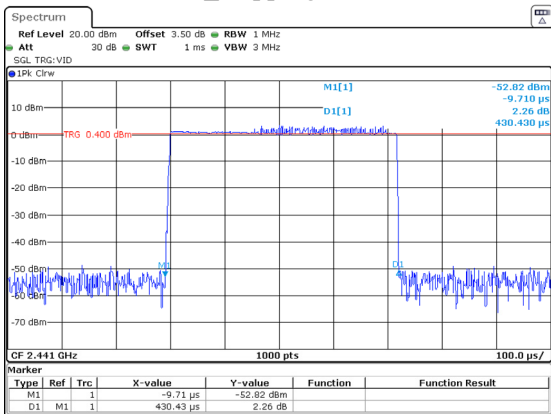
2DH1_Hopping 0.430ms
