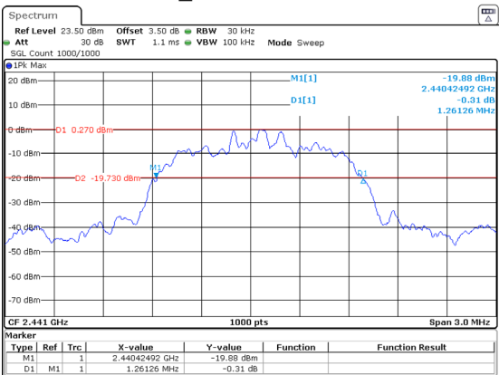
2DH1_Middle 1.261MHz
