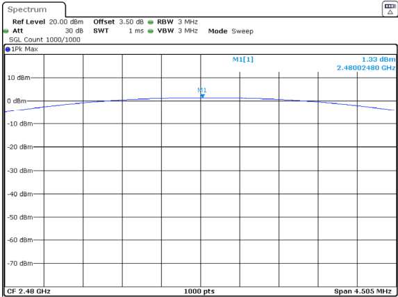
DH1_High 1.33dBm
