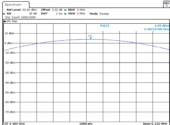
3DH1_Low 3.99dBm
