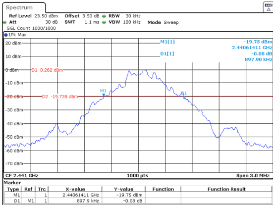
DH1_Middle 0.898MHz
