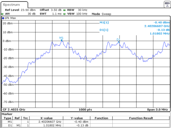
DH1_Low 1.018MHz
