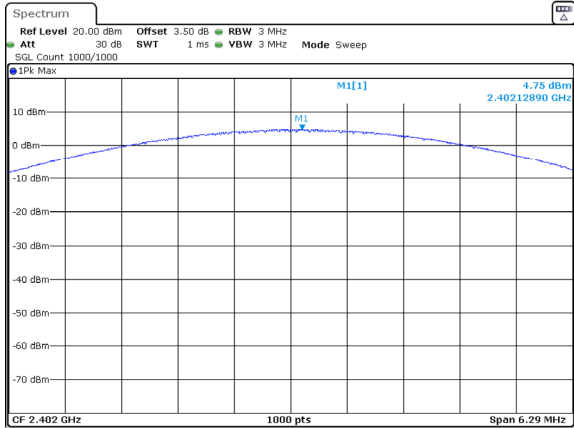
2DH1_Low 4.75dBm
