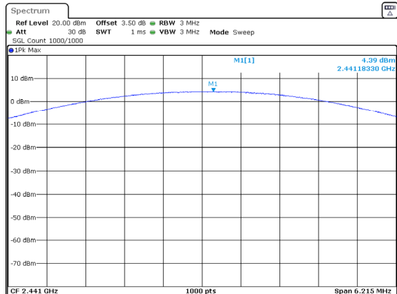
3DH1_Middle 4.39dBm
