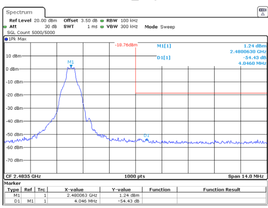
DH1_High
