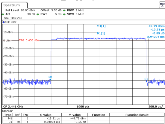
2DH5_Hopping 2.943ms
