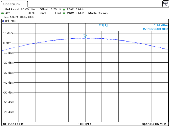
2DH1_Middle 5.14dBm
