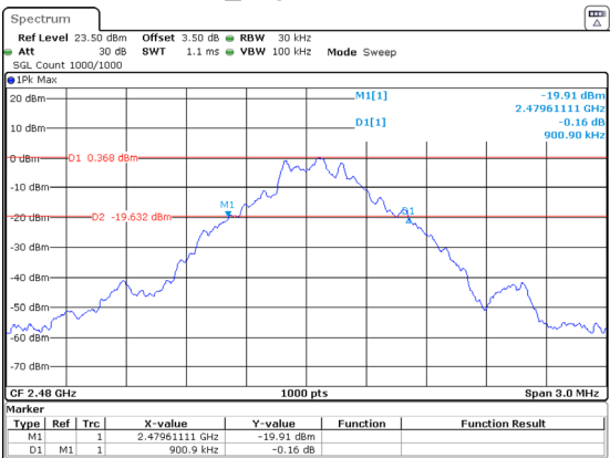
DH1_High 0.901MHz
