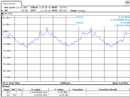
DH1_Middle 1.021MHz
