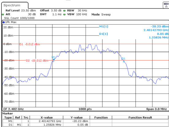
2DH1_Low 1.258MHz
