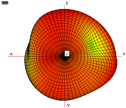
3D Radiation Pattern @ 2400 MHz
