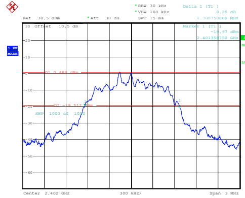
2DH1_Low 1.309MHz
