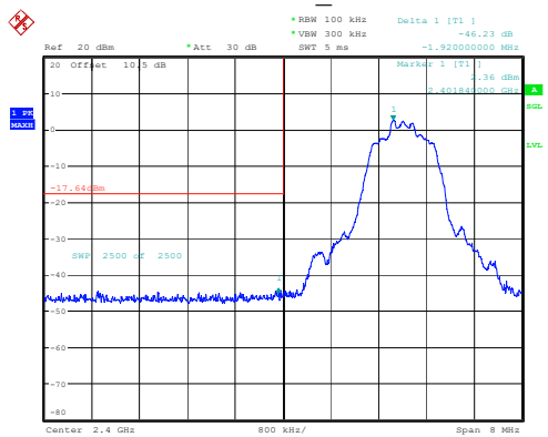
2DH1_Low
