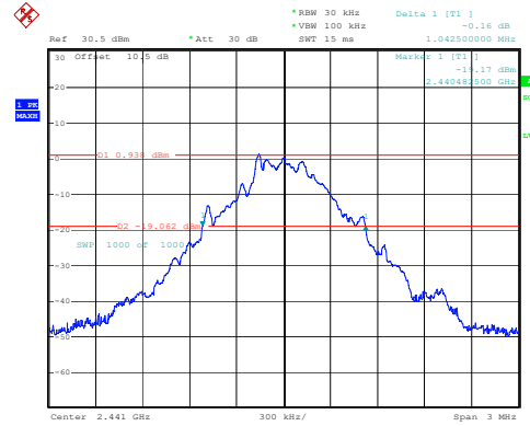
DH1_Middle 1.043MHz
