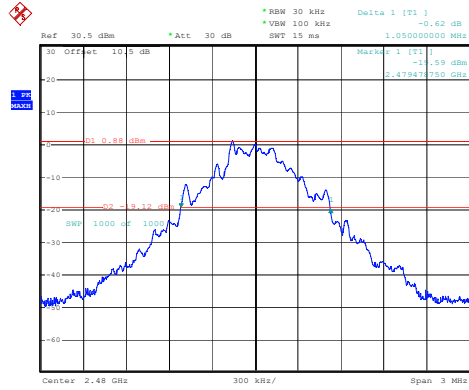
DH1_High 1.050MHz
