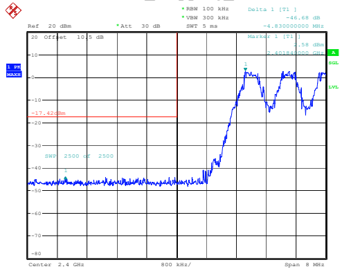
DH1_Hopping_Lower
