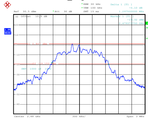
2DH1_High 1.297MHz
