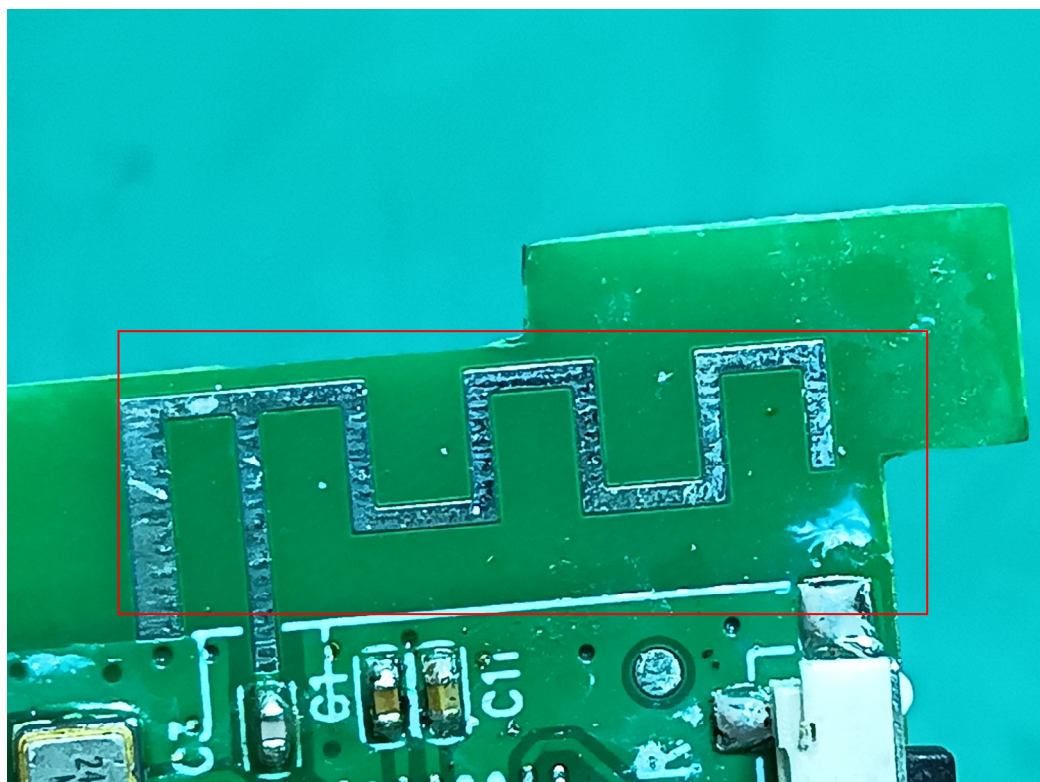
BT Antenna
