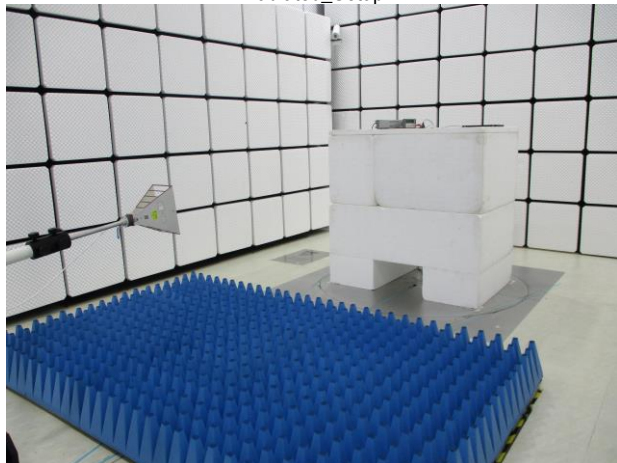
Radiated_Setup
