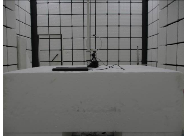
FCC_15_247_Radiated_spot check_Setup
