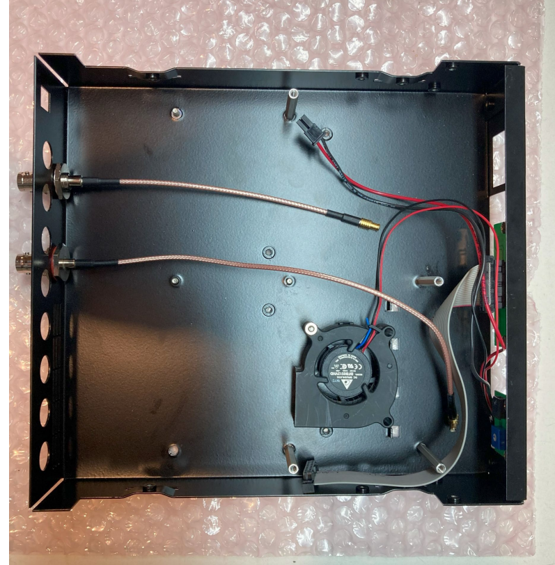
CHASSIS INTERNAL
