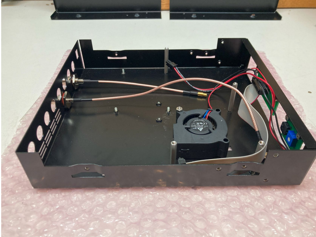
CHASSIS INTERNAL
