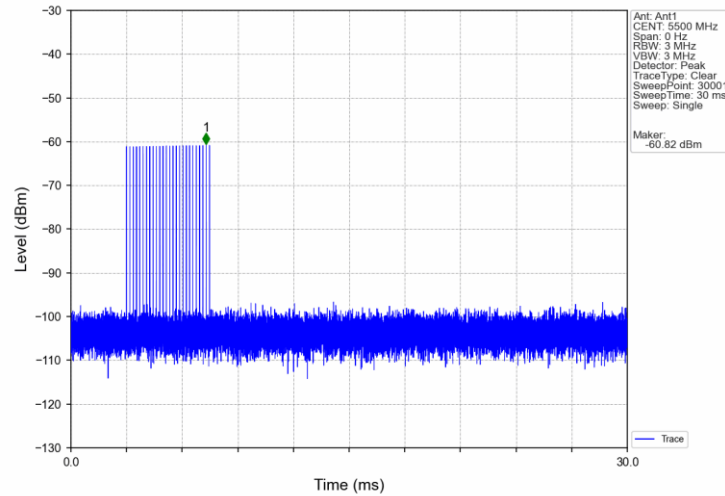
Signal Calibration 802.11a 2C 5500MHz RadarType3 Trial0
