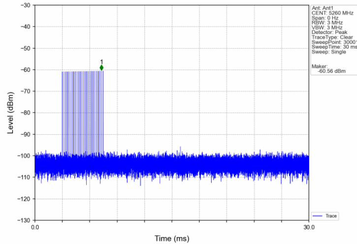
Signal Calibration 802.11a 2A 5260MHz RadarType3 Trial0
