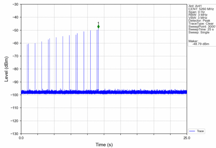
Signal Calibration 802.11a 2A 5260MHz RadarType5 Trial0
