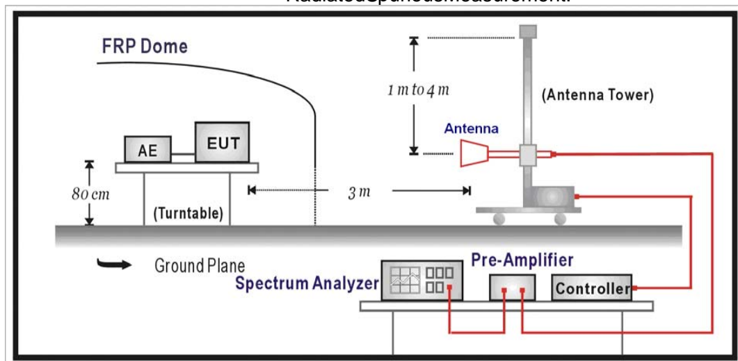
RadiatedSpuriousMeasurement:
