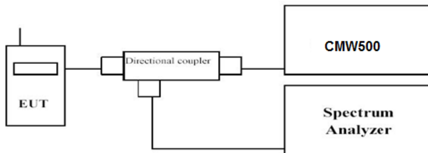
ConductedSpuriousMeasurement:
