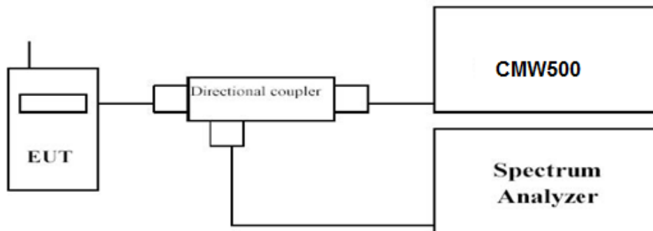
ConductedSpuriousMeasurement:
