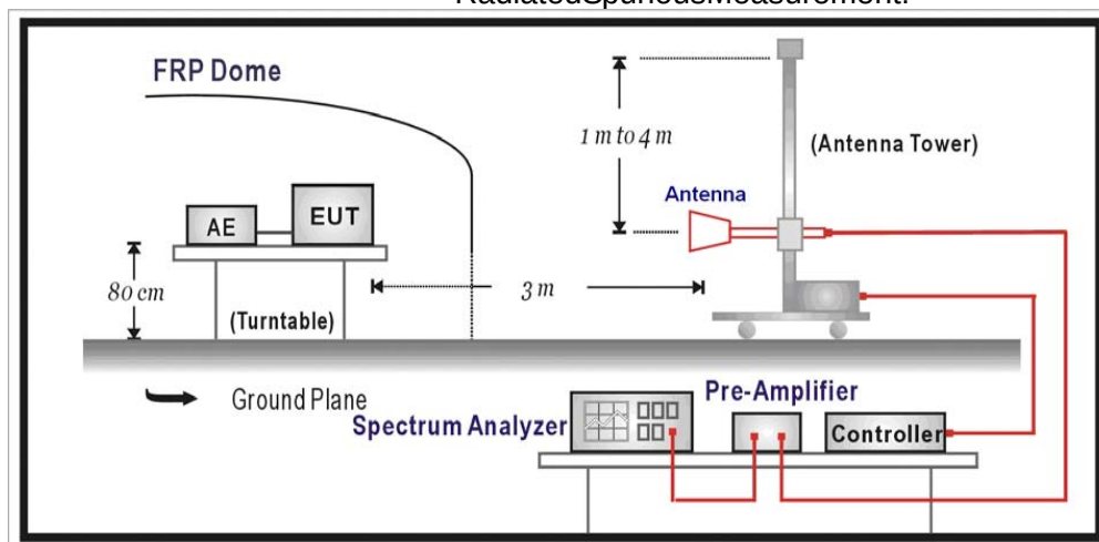
RadiatedSpuriousMeasurement:
