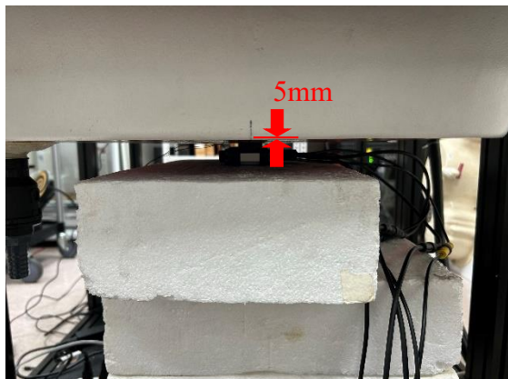
Photograph 11. Body, Back Surface, 5mm
