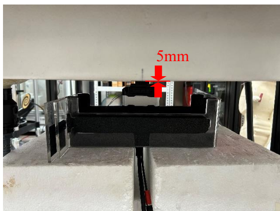
Photograph 13. Body, Top Edge, 5mm
