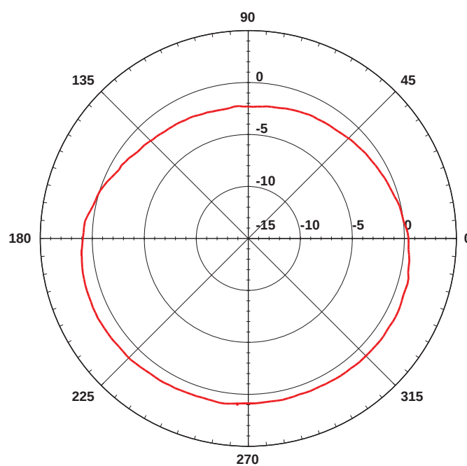
Total field (dBi)
