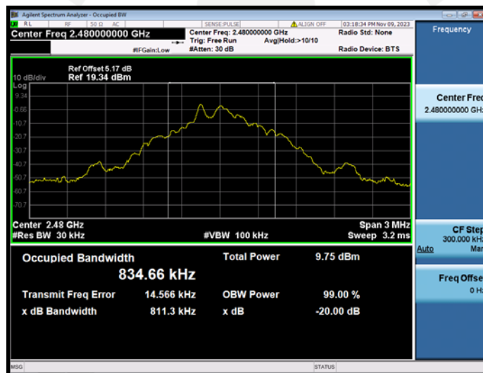
GFSK(1-DH1) 2480MHz
