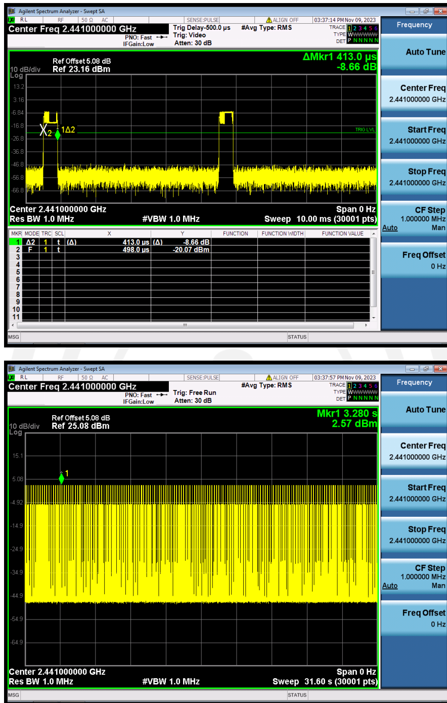
GFSK (1-DH1) 2441MHz
