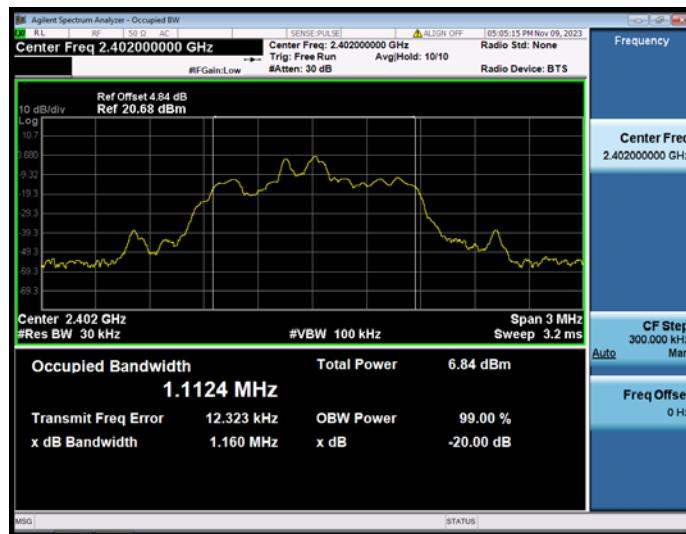
8DPSK (3-DH1) 2402MHz
