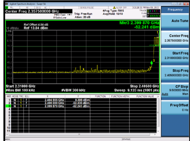
GFSK Hopping
