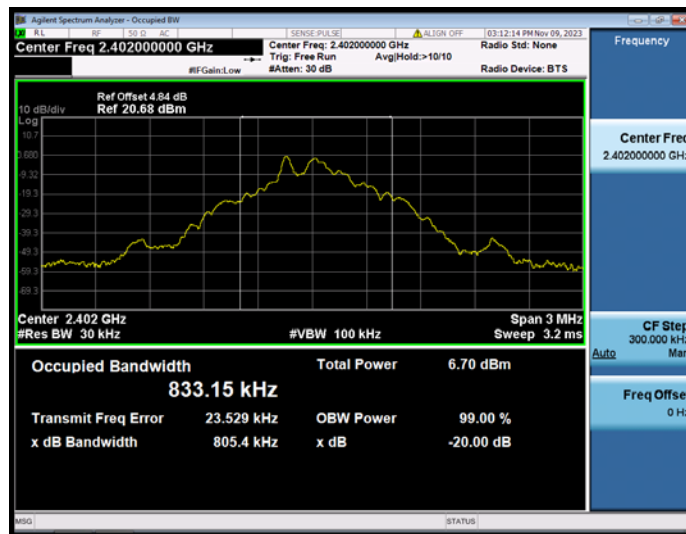
GFSK(1-DH1) 2402MHz
