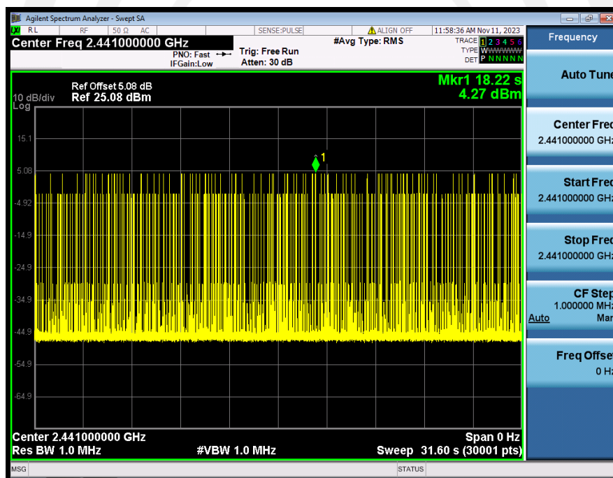
π/4-DQPSK (2-DH5) 2441MHz
