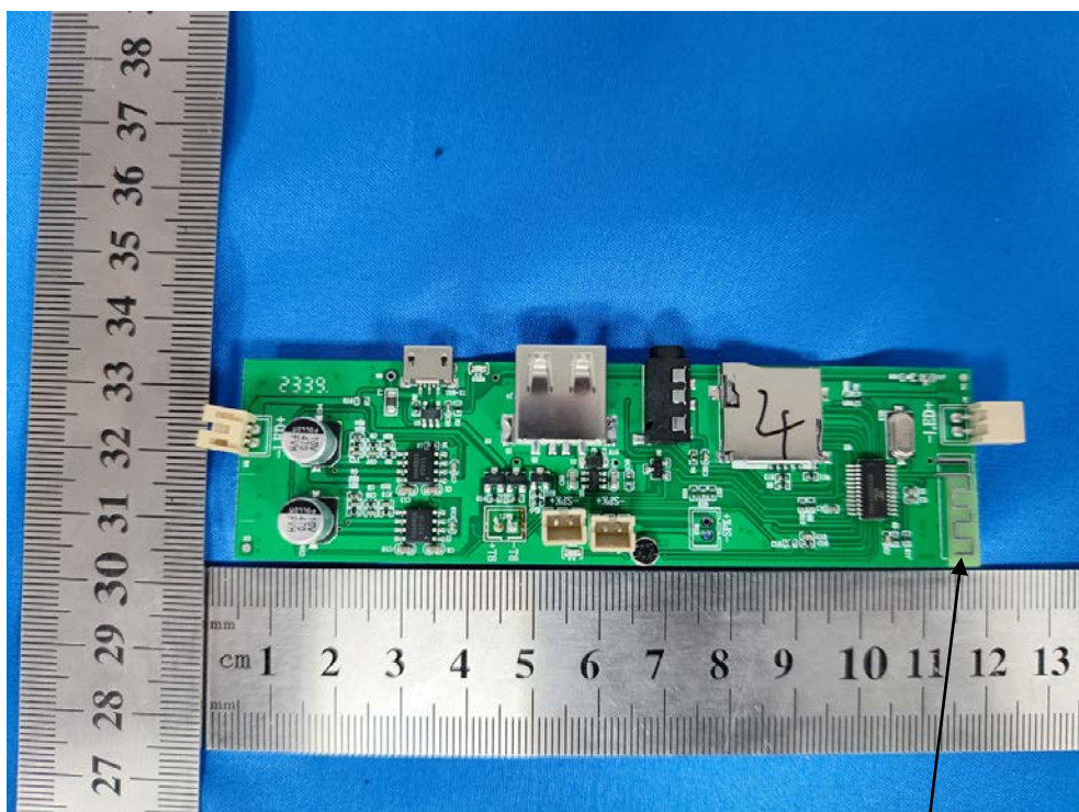
Antenna Location
