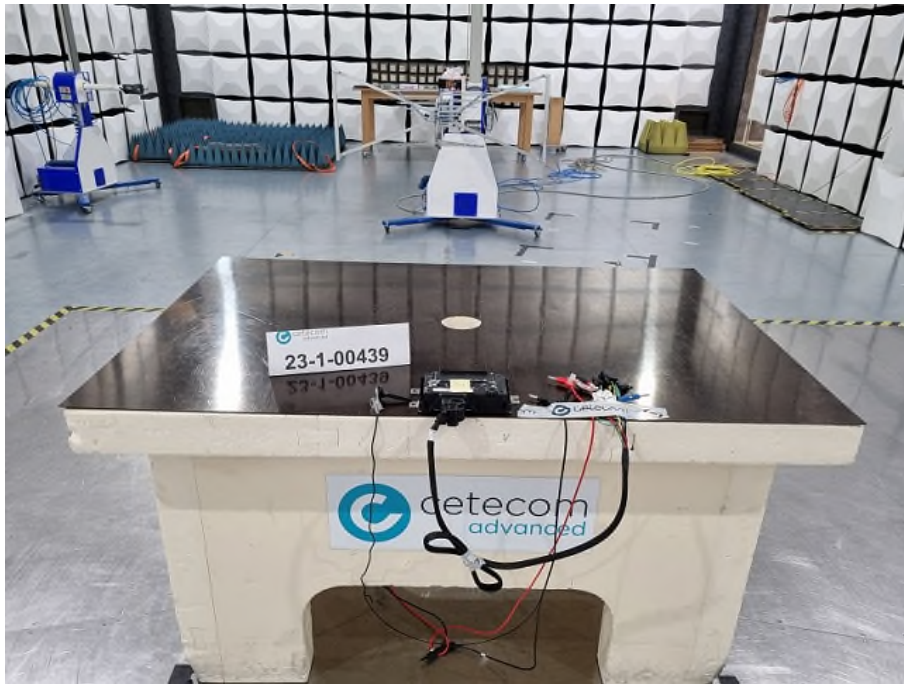
Photograph 3 : Measurements < 1GHz in SAC, rear side view
