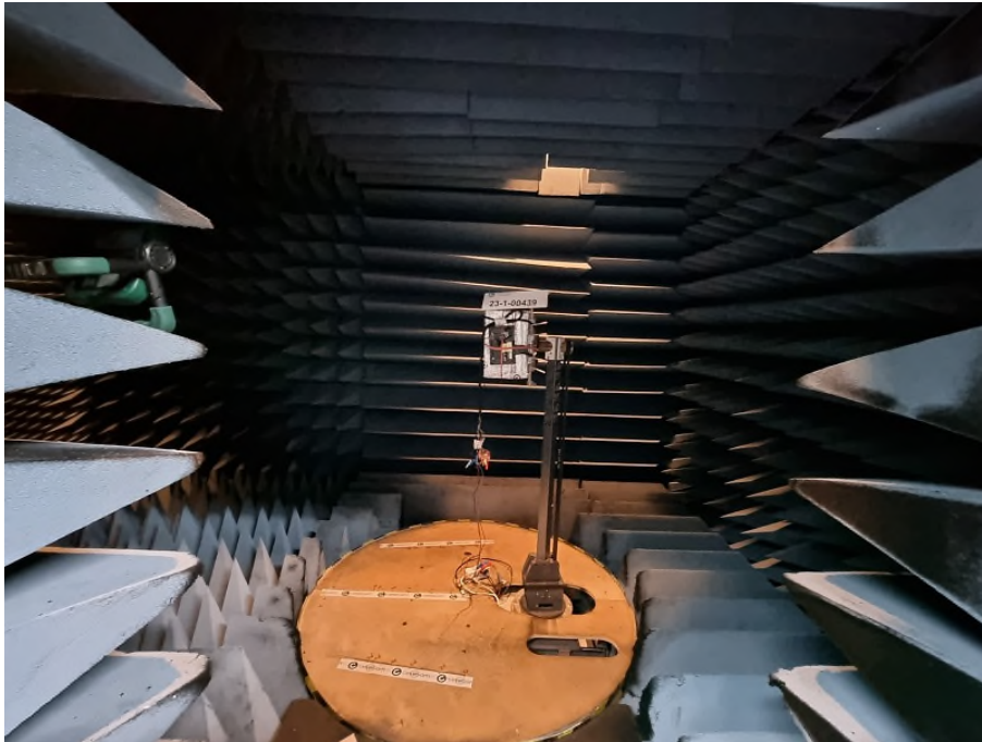
Photograph 5 : Measurements > 1GHz in FAC, overview
