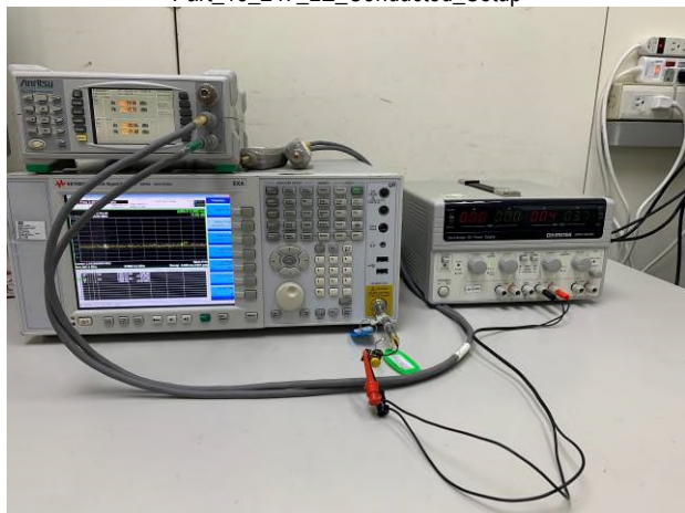
Part_15_247_LE_Conducted_Setup
