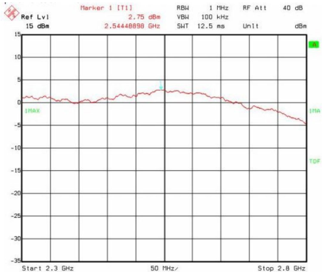
Figure 8:OUTPUT POWER,esp32
