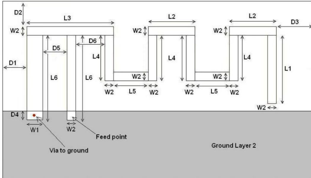
Figure 2: Antenna Dimensions ( mm)
