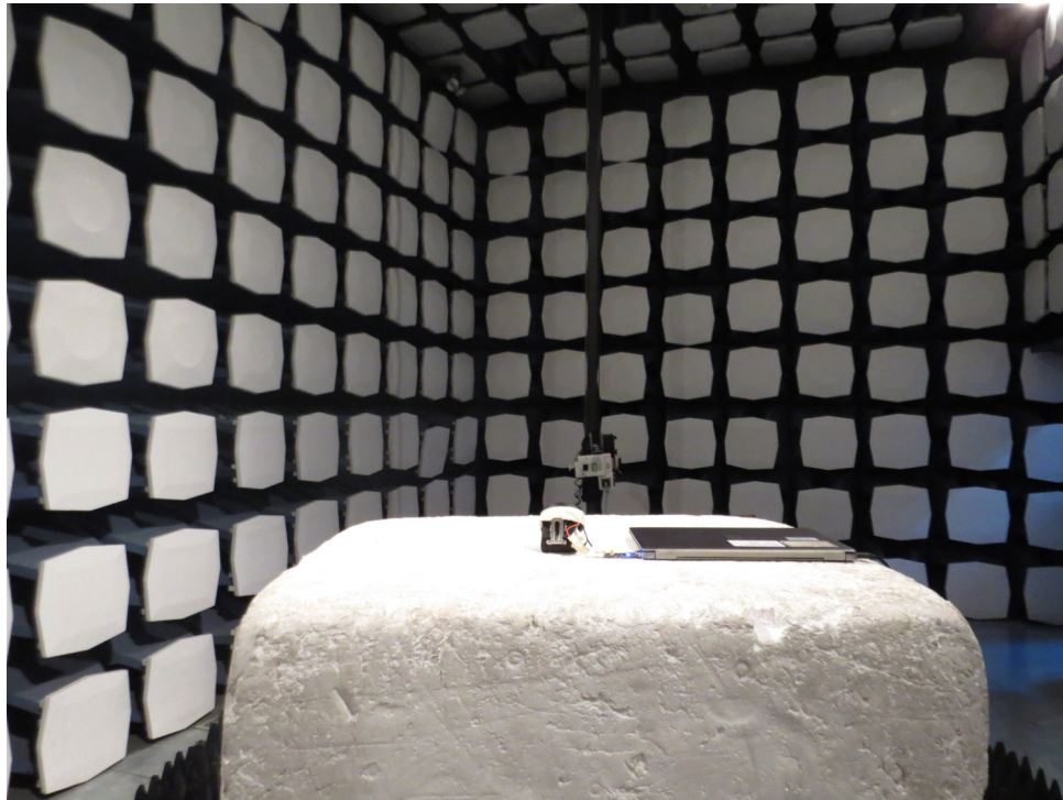
Picture 1 Radiated Emission Test Setu
