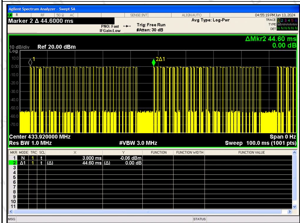
T_{on} + T_{off}
