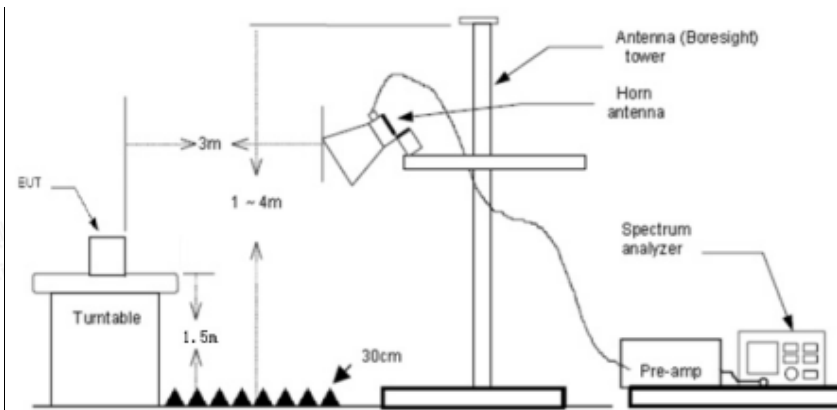
Above 1GHz
