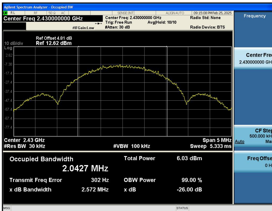
99%_Occupied_Bandwidth_NVNT_ANT1_2Mbps_2430
