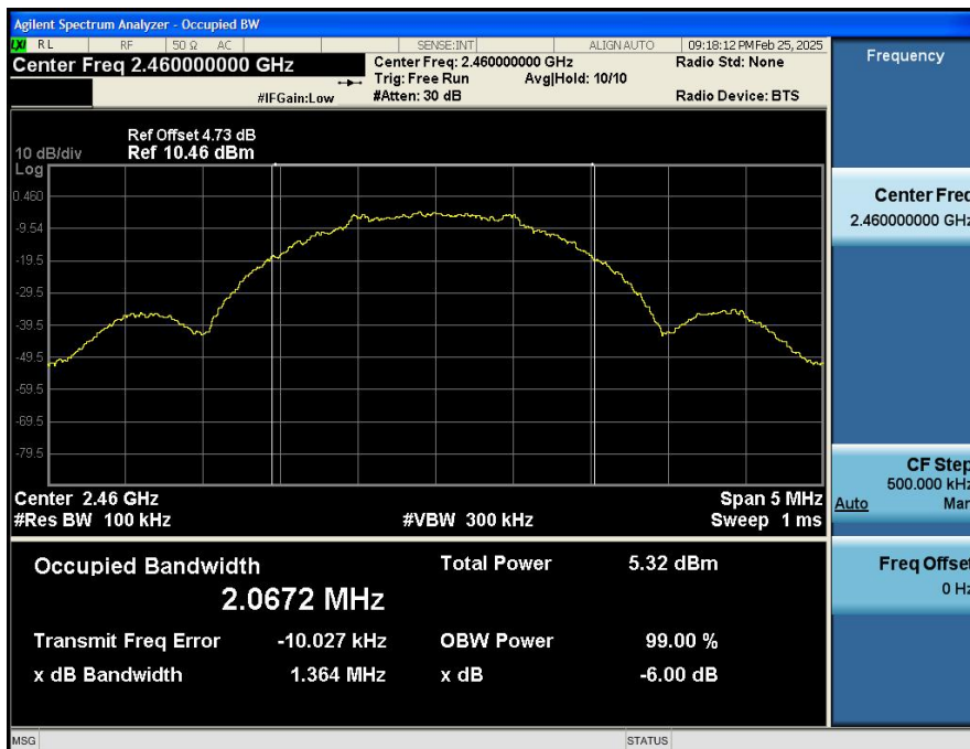
-6dB_Bandwidth_NVNT_ANT1_2Mbps_2460
