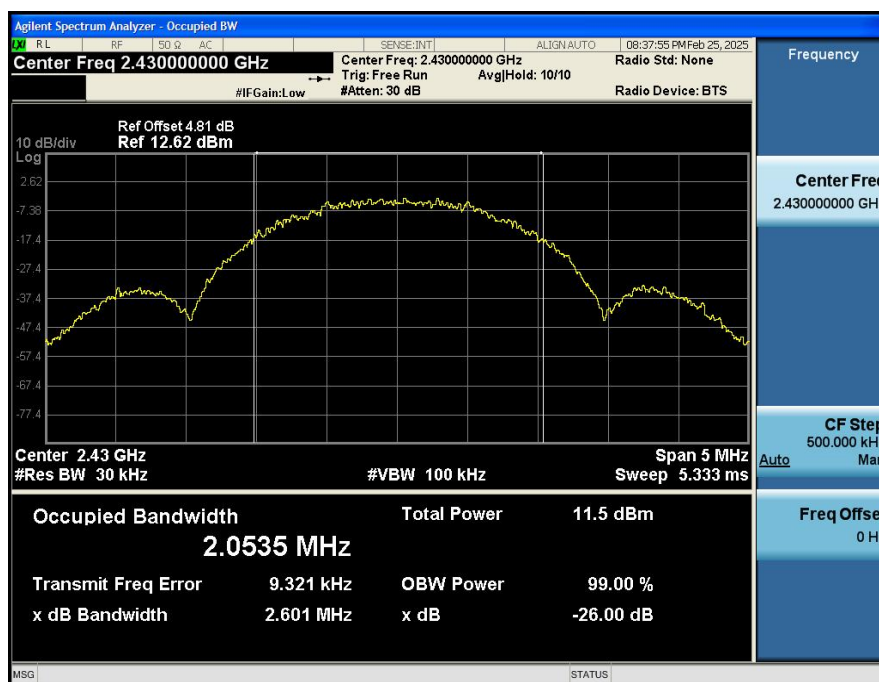
99%_Occupied_Bandwidth_NVNT_ANT1_2Mbps_2430
