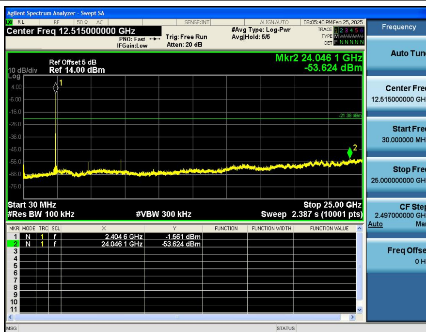
2_Spurious_Emission_NVNT_ANT1_2405
