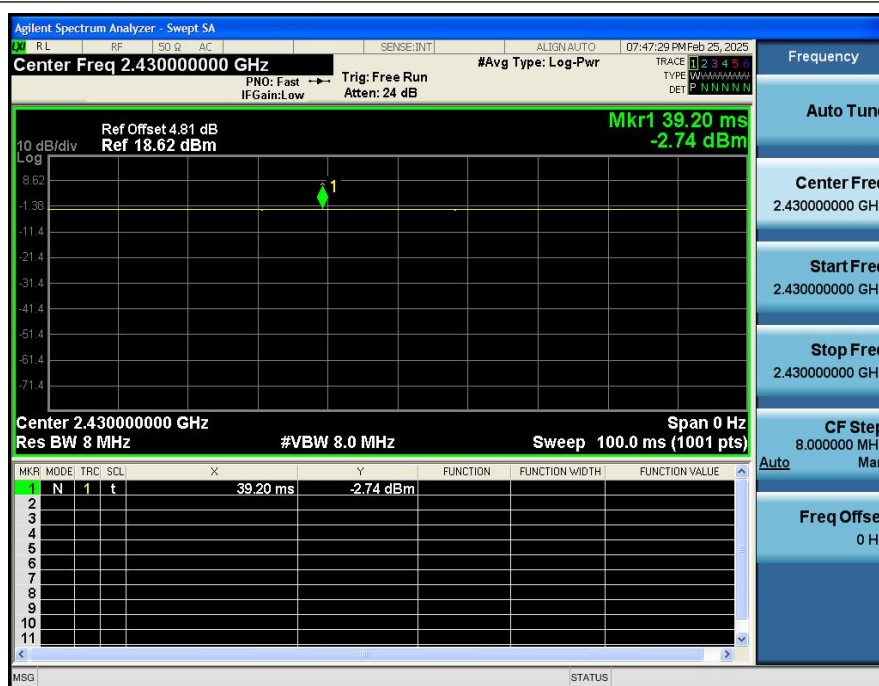
Duty_Cycle_NVNT_ANT1_2430
