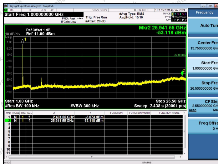
2.4G-Ant1-2402-1000~26500-PASS
