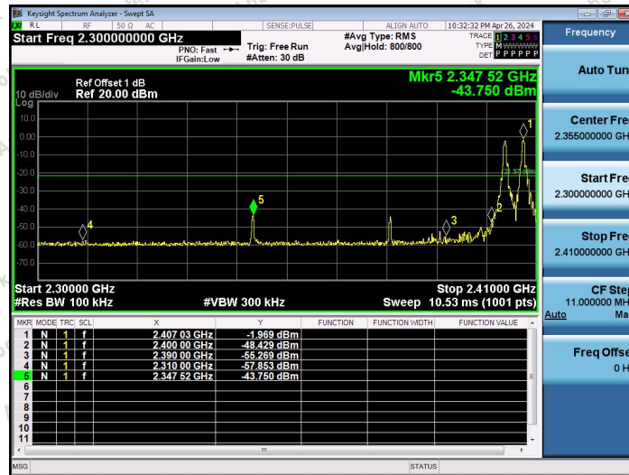
2.4G-Ant1-Hop_2402-PASS
