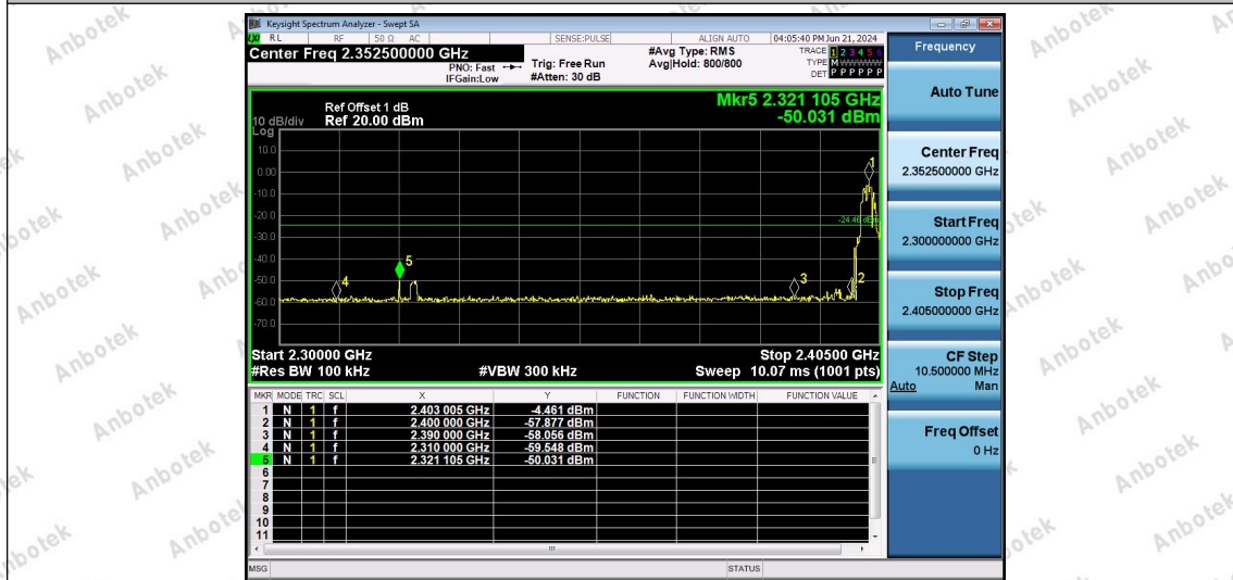
2.4G-Ant1-Hop_2402-PASS
