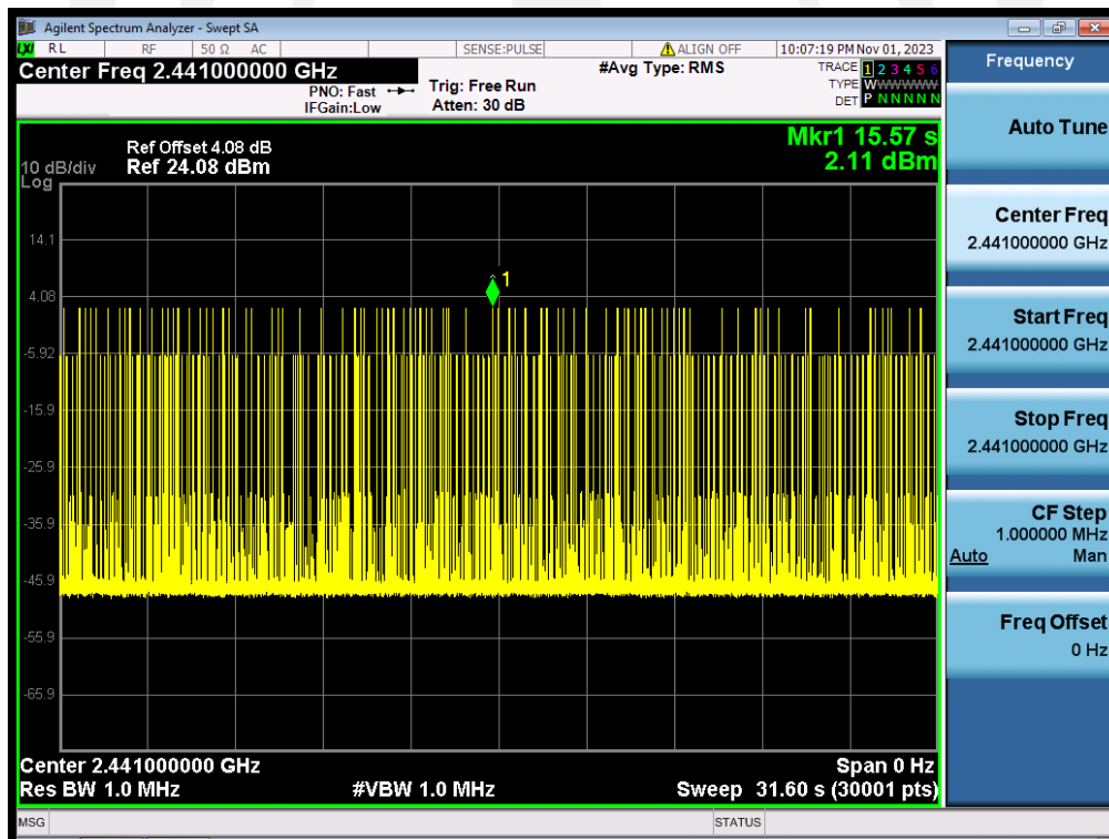
GFSK (1-DH5) 2441MHz
