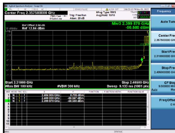
GFSK Hopping
