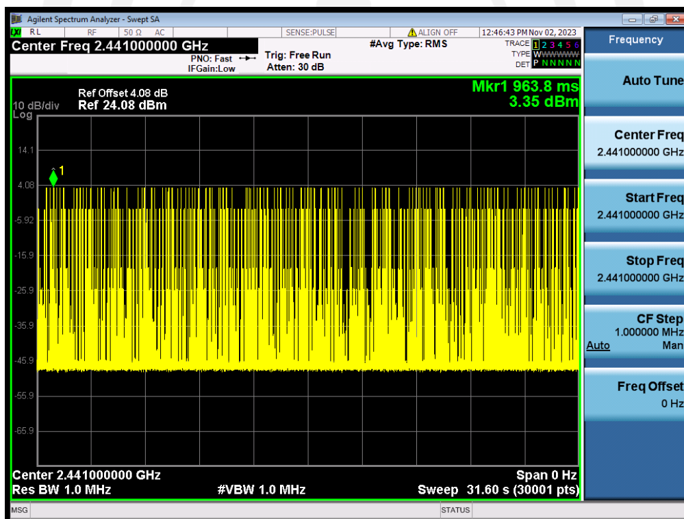
8DPSK (3-DH3) 2441MHz
