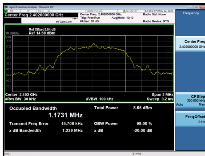
8DPSK (3-DH1) 2402MHz
