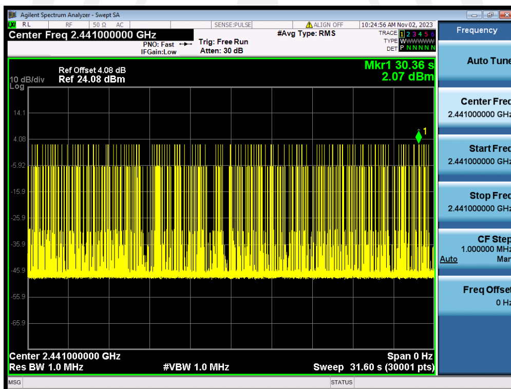
GFSK (1-DH3) 2441MHz
