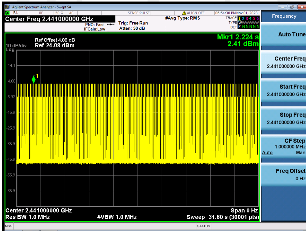
GFSK (1-DH1) 2441MHz
