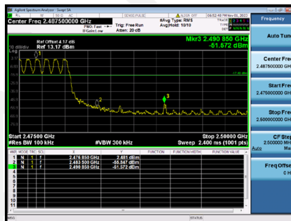
GFSK Hopping
