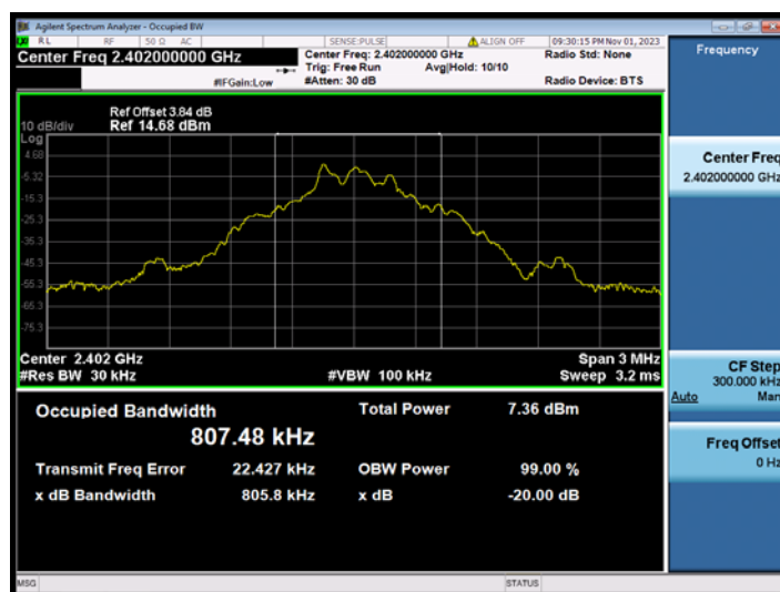
GFSK(1-DH1) 2402MHz
