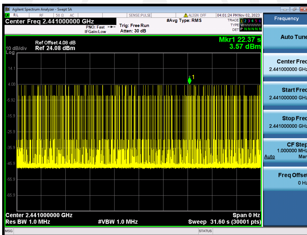
8DPSK (3-DH5) 2441MHz
