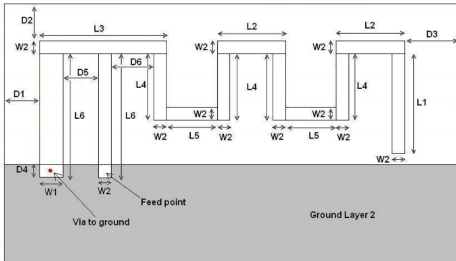
Figure 3: Antenna Dimensions
