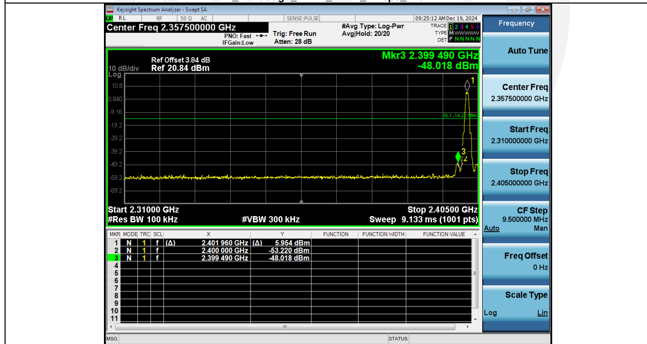
2 Bandedge_NVNT_ANT1_1Mbps_2402
