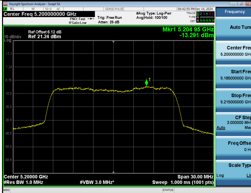
Power Spectral Density_NVNT_ANT1_802_11ac(VHT20)_5200
