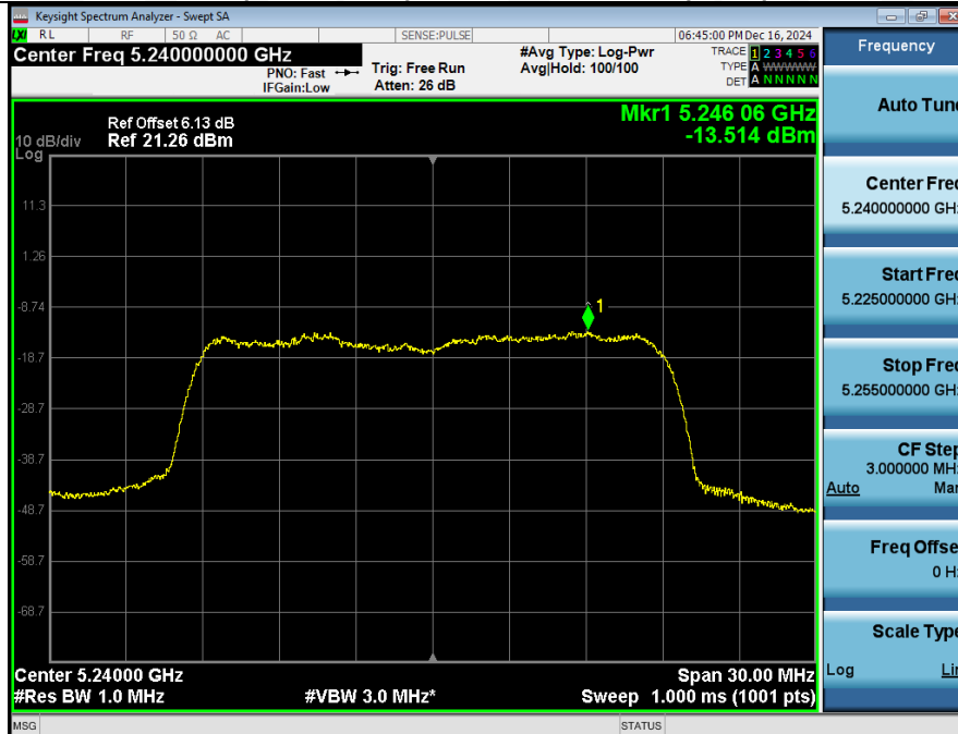
Power Spectral Density_NVNT_ANT1_802_11ac(VHT20)_5240
