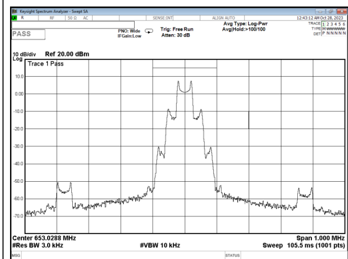
Channel 1 / 653.0288 MHz
