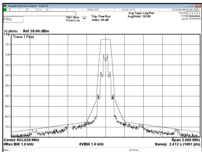
Channel 1 / 653.0288 MHz
