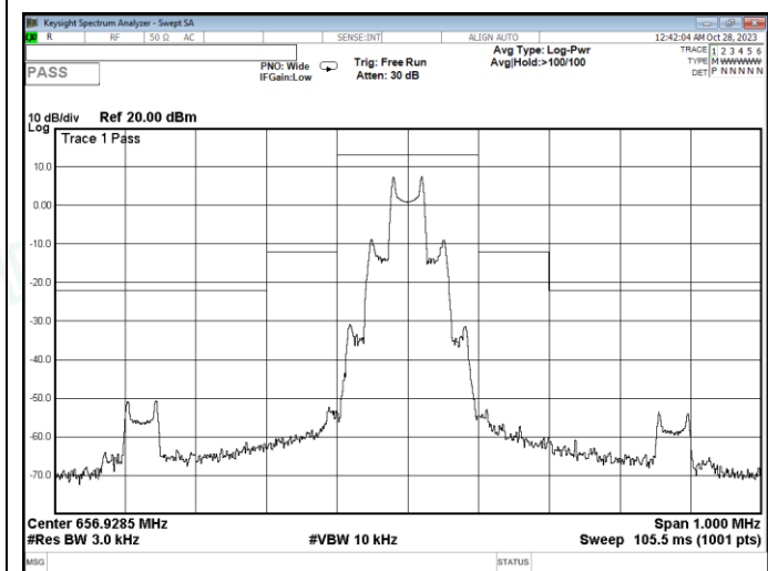
Channel 14 / 656.9285 MHz
