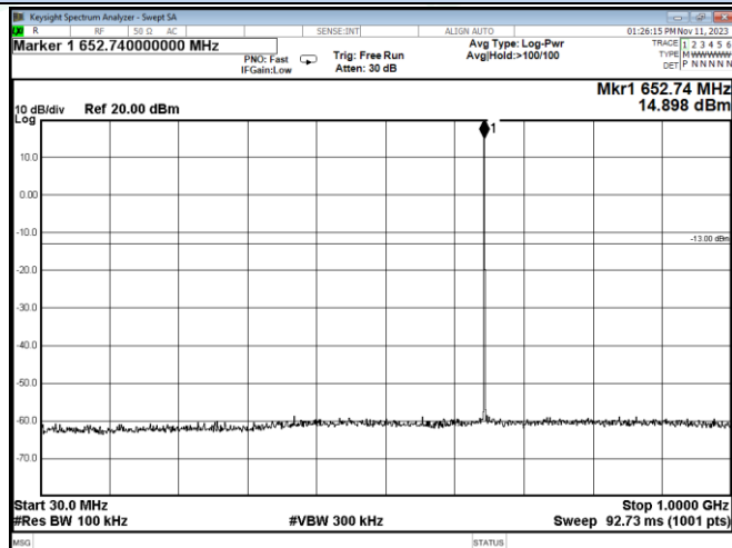
Channel 1 / 653.0288 MHz
