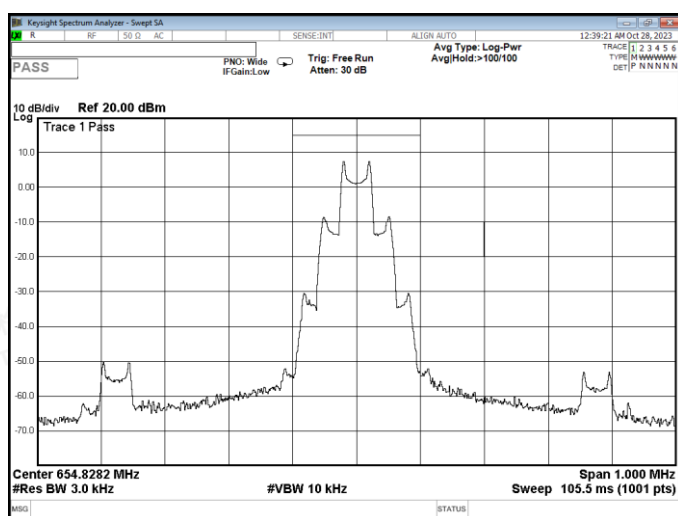
Channel 7 / 654.8282 MHz
