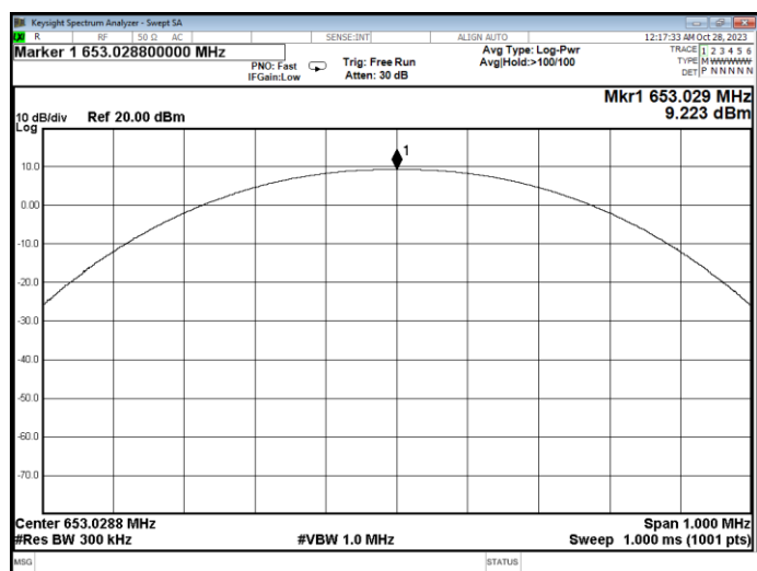
Channel 1 / 653.0288 MHz
