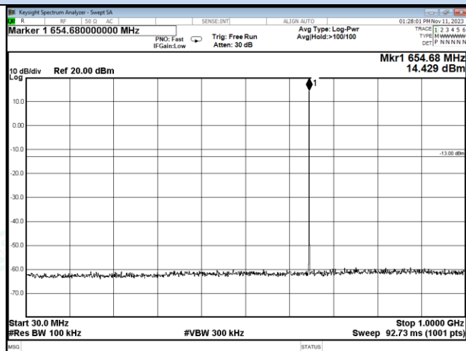
Channel 7 / 654.8282 MHz
