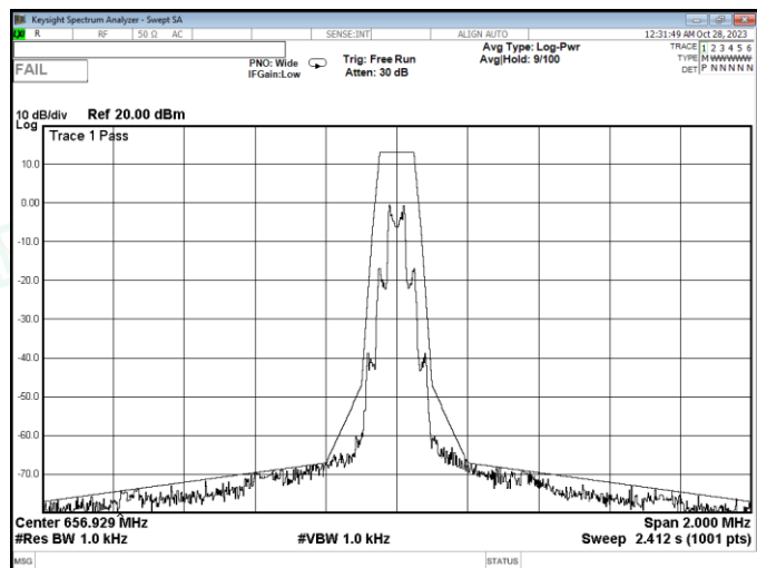
Channel 14 / 656.9285 MHz
