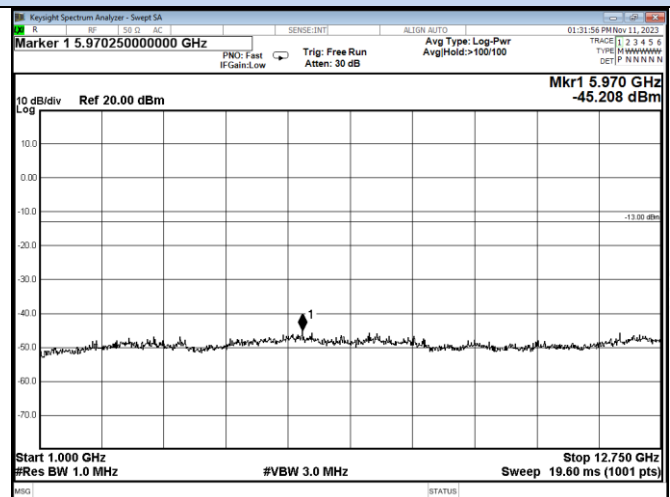
Channel 7 / 654.8282 MHz
