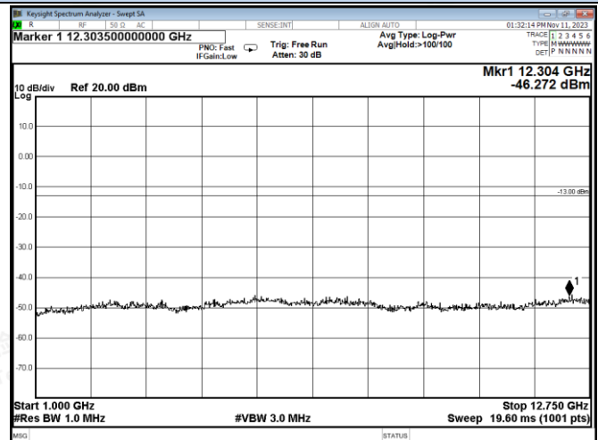
Channel 1 / 653.0288 MHz
