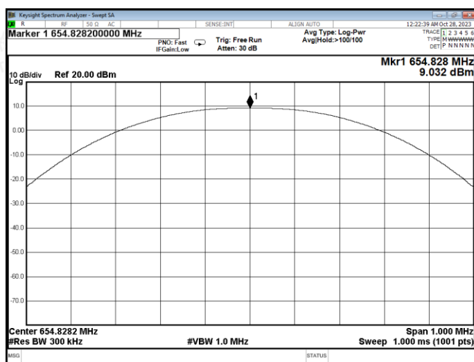
Channel 7 / 654.8282 MHz
