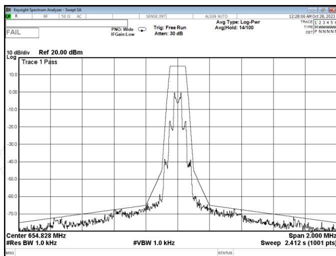
Channel 7 / 654.8282 MHz
